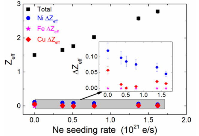
FIG. 11. Incremental Z_{\text{eff}} deliver from Ni, Fe and Cu using VUV diagnostic in comparison on total effective charge Z_{\text{eff}} determined form visible Bremsstrahlung measurements as a function of Ne seeding rate.
