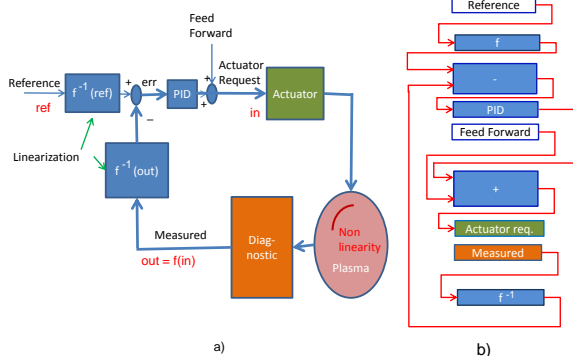
Fig.1 a) A simple closed loop algorithm with compensation for static nonlinearity. b) Schematic illustration of the implementation of this controller in the RTCC language.
