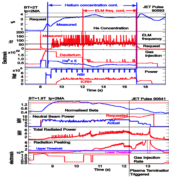
Fig.7 a) simultaneous control of the ELM frequency and He 3 concentration by injection of Deuterium and He 3 gas. b) simultaneous operation of a normalised beta controller by NBI and a bang/bang control scheme aimed at reacting to radiation peaking. At 12.2 seconds a discharge termination is triggered due to the detection of MHD activity.
