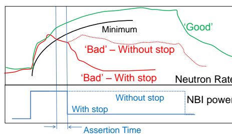
Fig.2 ‘Dud’ detection. When the neutron production is deemed unsatisfactory, the pulse is terminated.
