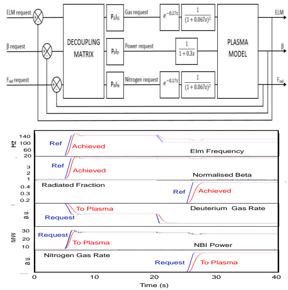
Fig. 8 MIMO controller: a) 3x3 control block diagram the decoupling matrix is the inverse of the steady state plasma matrix in the linearization point. b) Simulation of 3x3 control
