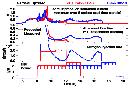
Fig.5 Closed loop detachment control without a) and with b) compensation for the non-linearity seen in figure 4.
