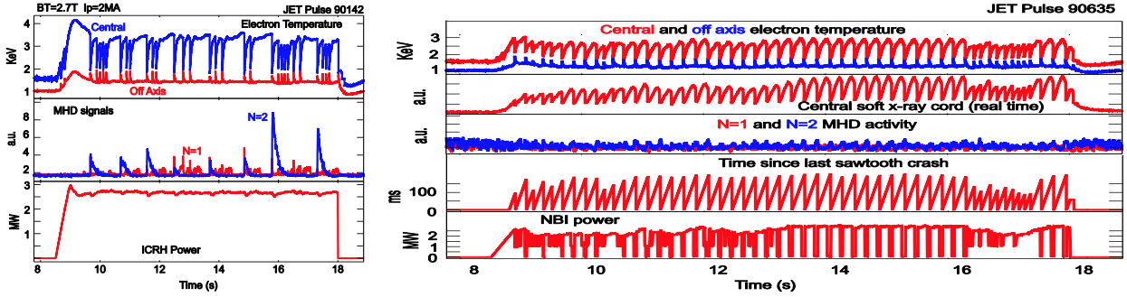
Fig.3 Sawtooth and N=2 activity for two discharges: 'a) Constant ICRH power. Long sawteeth trigger N=2 NTMs. ( 90142); b) Effective sawtooth pacing leading to the avoidance of NTMs.
