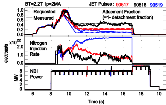
Fig.5 Closed loop detachment control without a) and with b) compensation for the non-linearity seen in figure 4.
