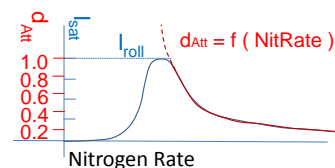
Fig.4 Sketch showing attachment fraction d_{Ait} = I_{sat}/I_{roll} as a function of input gas flow rate (blue) and an exponential curve matching this for nitrogen rates beyond the rollover (red).
