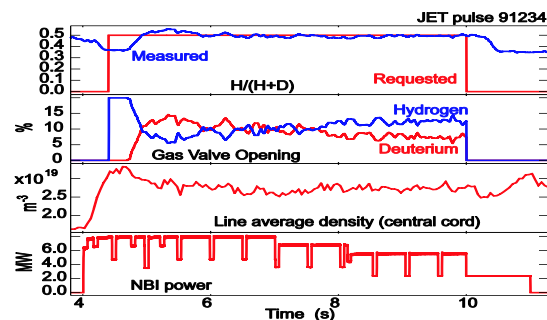
Fig.6 Hydrogen-Deuterium mixture control. (#91234). The controller compensates for the disturbance introduced by variations in the deuterium neutral beam power.
