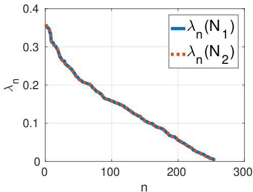
Figure 6: The sorted eigenvalues (with the absolute values shown on the plot) of the operators N_1 and N_2 defined in Eq. (4.3) coincide, confirming the consistency of our solver. Here, the case corresponding to N_p = 10^4 “polarisation-density particles” and adiabatic electrons is shown. Note the linear scale on the vertical axis of this plot (the logarithmic scale has been used in Fig. 5).
