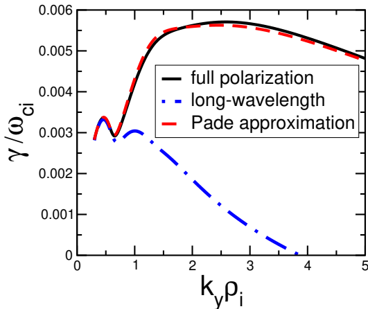
Figure 2: Comparison of the ITG growth rates computed using the full polarisation density, the Padé approximation and the long-wavelength approximation. The local dispersion relation in slab geometry (Mishchenko et al. 2018) has been solved numerically.
