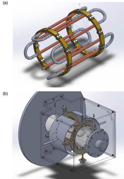
Figure 4: Helicon plasma sources: (a) drawing of the resonant antenna with main elements: capacitors assemblies, copper rods, and cooling water circuit; (b) installation of the antenna on the end flange of the RAID device; the two semi-cylindrical metallic screens allow fine tuning of the resonant frequency.
