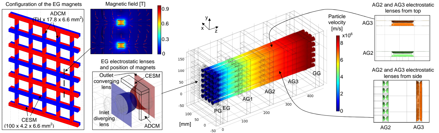
Figure 5: Overview of the self-consistent electrostatic-magnetic-particle tracking model of the DEMO NBI accelerator. The model includes all the grids, with circular apertures in the first three grids, slotted apertures in the AG2 and frame-like apertures in the AG3 and GG. As a consequence, the electrostatic lenses have a different shape in the different grids. The EG features two sets of permanent magnets: CESH (to suppress the co-extracted electrons) and ADCM (to compensate for the alternate deflection of the negative ions generated by the CESH).
