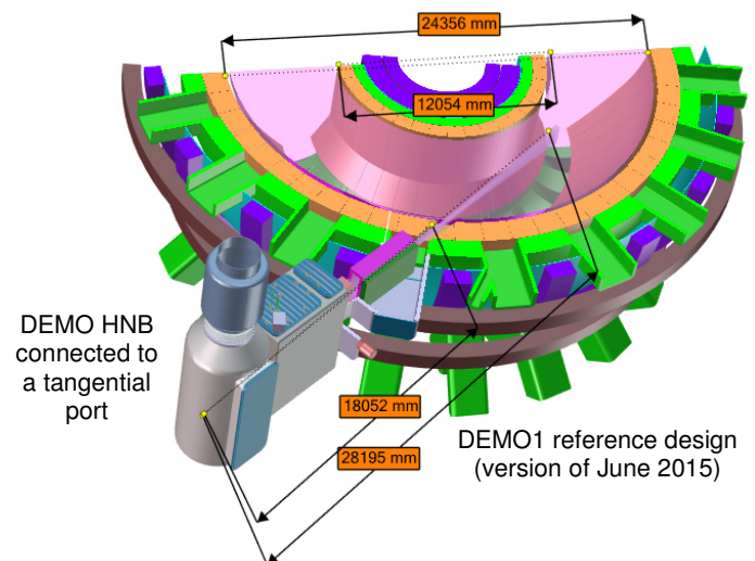
Figure 1: Integration of the Heating Neutral Beam in the DEMO1 pre-conceptual design.
