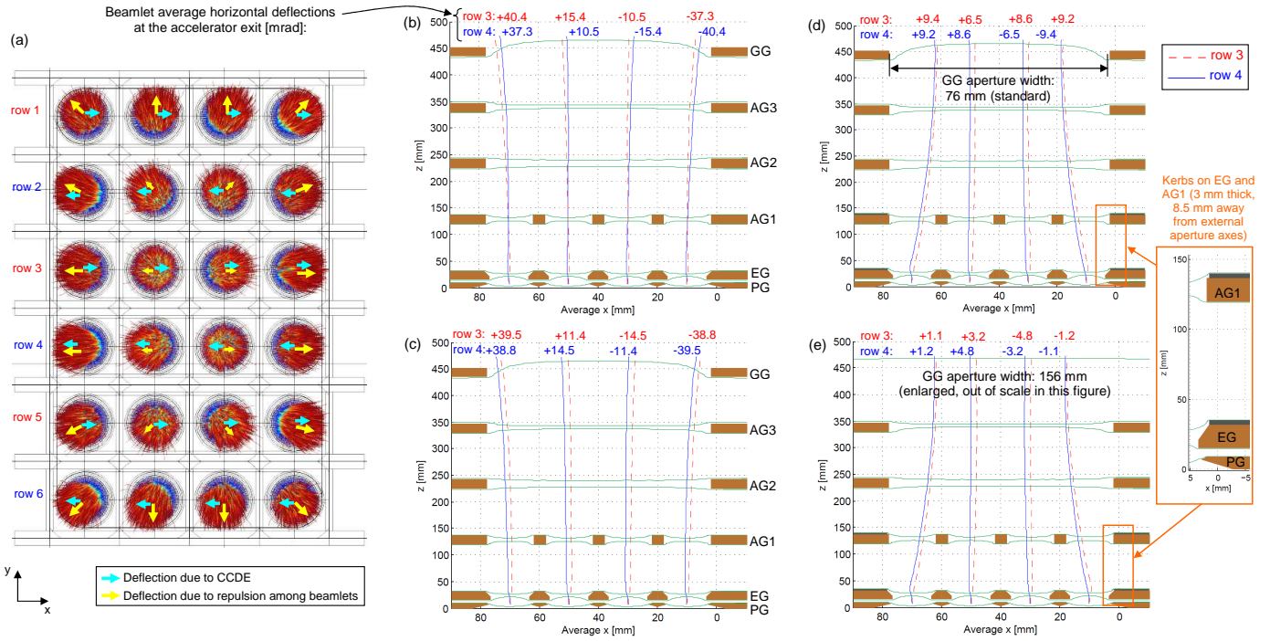
Figure 7: Main result of the full model with 4x6 apertures: (a) Trajectories seen from downstream, where the effect of the repulsion among beamlets and CCDE can be clearly observed (here, the case without ADCM is considered); (b) beamlet trajectories without ADCM; the horizontal residual deflections at the exit (reported for beamlet rows 3 and 4) are influenced by the repulsion among beamlets plus CCDE; (c) beamlet trajectories with 2 mm thick ADCM; CCDE is significantly reduced; (d) beamlet trajectories with 2 mm thick ADCM and kerbs; repulsion effect is reduced (e) beamlet trajectories with 2 mm thick ADCM, kerbs and enlarged GG aperture; repulsion effect is almost completely compensated, as the eight beamlets are now almost parallel to the beam axis at the accelerator exit. The main electrostatic lenses are plotted in green.
