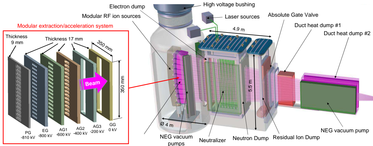
Figure 2: Overview of the DEMO NBI with the main components and a sketch of the grids of the modular extraction/acceleration system.
