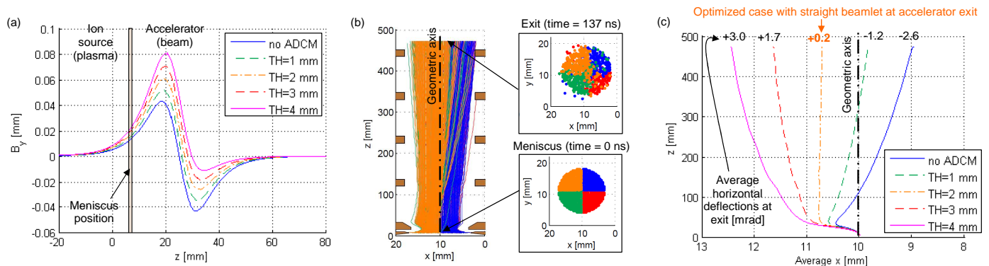
Figure 6: Main results of the single beamlet simulation: (a) magnetic field profile along the aperture axis with different values of the ADCM thickness; (b) particle trajectories in the case with no ADCM (the particles from the four quarters of the meniscus have a different color so that the deflection effect is more visible); (c) particle average trajectory with different values of the ADCM thickness. It can be observed that the case with an ADCM thickness of 2 mm provides an almost perfect compensation of the CCDE.
