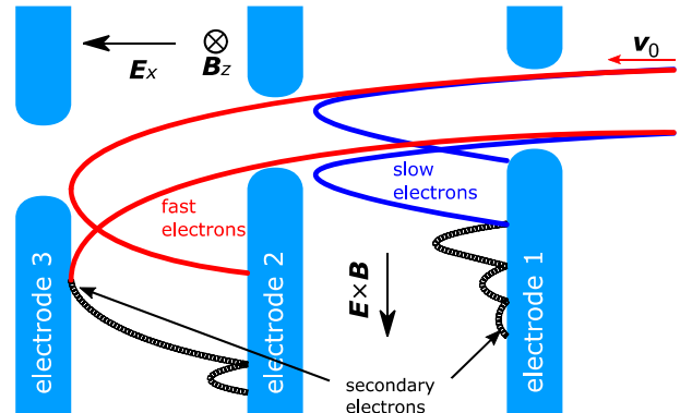
Fig. 6. E \times B concept for multi-stage depressed collector technologies as proposed in [34, 35]. The secondary electrons are always guided towards the electrodes of the collector (picture by C. Wu).
