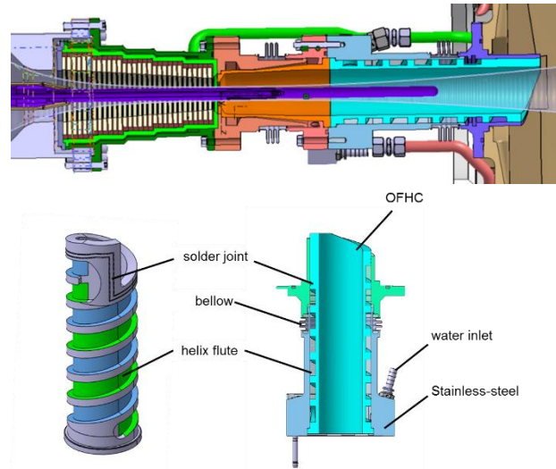
Fig. 4. Cooling concept for the key components beam tunnel, cavity and launcher (top), detailed cooling concept for the launcher (bottom).
