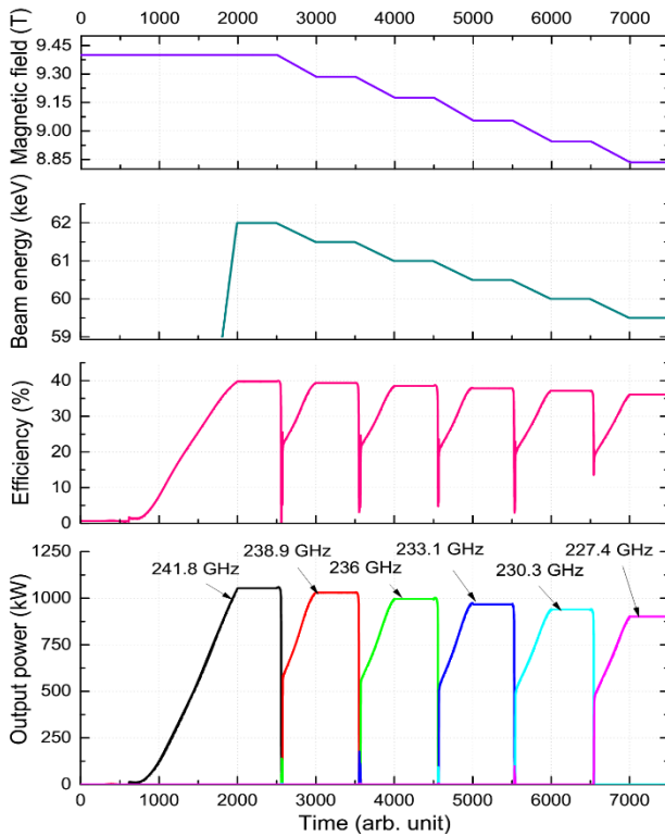
Fig. 3. Calculated magnetic field, beam energy, efficiency and output power for frequency step-tuning of the 236 GHz hollow-cavity gyrotron.
