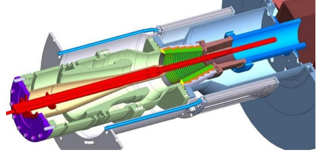
Fig. 1. 3D image of a typical coaxial insert (red) within a coaxial-cavity gyrotron.
