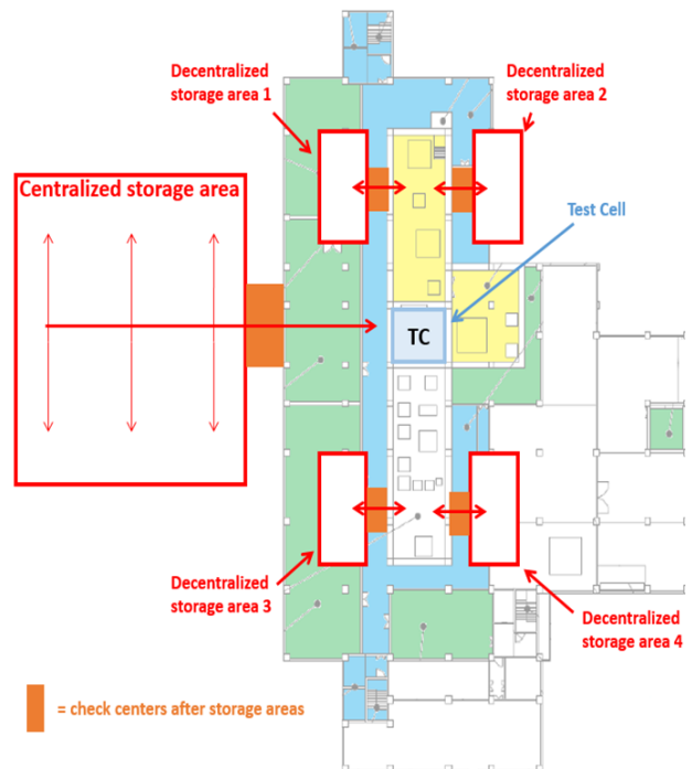
Fig. 5. Decentralized and centralized storage areas in the DONES facility (top view) [9]
