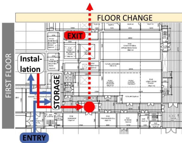
Fig. 2. Path of Beam Dump Cartridge through building.
