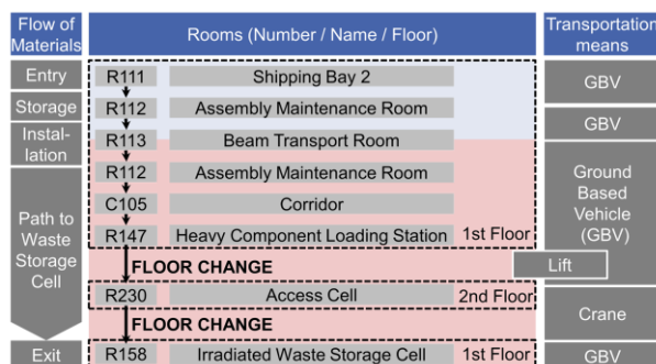
Fig. 1. Example Flow Chart: Beam Dump Cartridge [3].
