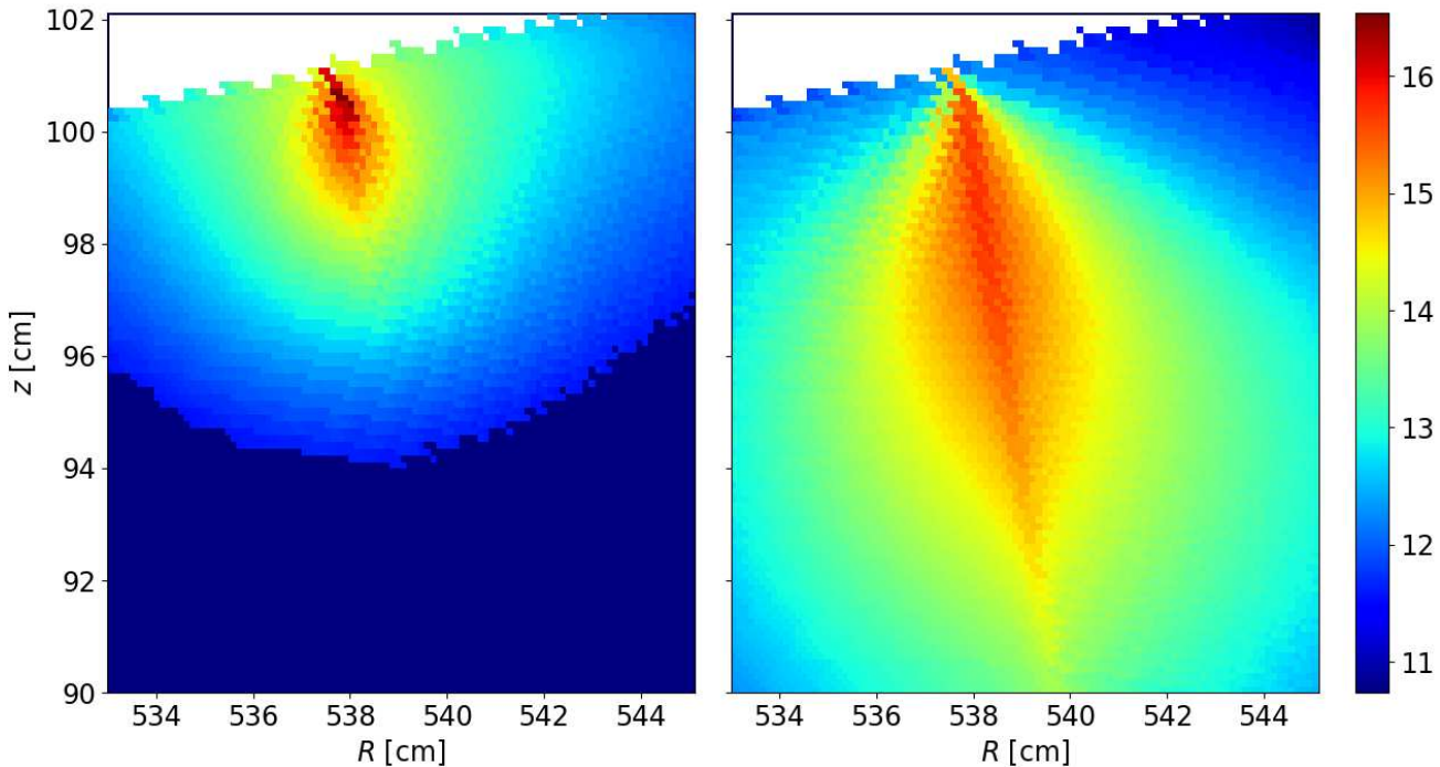
Figure 7. Decadic logarithm of the 706.5 nm line emissivity, \log_{10}(\varepsilon [1/\text{s}/\text{cm}^3]) , in the poloidal plane. Left – P_{\text{SOL}} = 10 MW and \langle n_e \rangle_{\text{LCFS}} = 5 \times 10^{13} \text{ cm}^{-3} , right – P_{\text{SOL}} = 1 MW and \langle n_e \rangle_{\text{LCFS}} = 5 \times 10^{12} \text{ cm}^{-3} . p-He elastic scattering included, formulation I, recombination neglected. Contrast limited to 10^5 , \dot{N} = 1.5 \times 10^{19} \text{ s}^{-1} .
