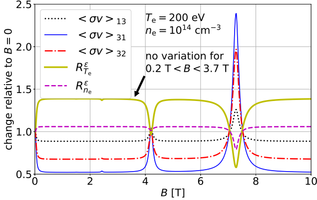
Figure 6. Dependence of coupling rate coefficients amongst ground and meta-stable states (see text), and of emissivity ratios (4) and (5) on the magnetic field, normalized to their value at 0 tesla.
