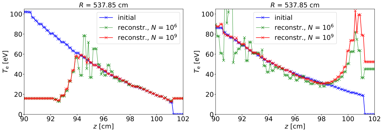
Figure 8. T_e reconstruction from the synthetic He beam diagnostic along vertical axis z (divertor at \approx 101 cm), according to the algorithm (see text). Left – reference profile from the average density case, right – low density case (see figure 3). Poloidal plane and radius fixed. N is the number of Monte Carlo test particles in the beam simulation.
