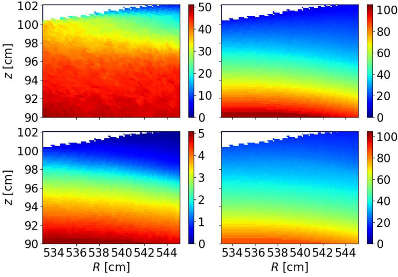
Figure 3. Background plasma density and temperature in front of the W7-X upper divertor, as generated by EMC3-EIRENE [33], depicted in the poloidal plane at the He nozzles' location. Left – n_e [ 10^{12} \text{ cm}^{-3} ], right – T_e [eV]. Top – medium density case with P_{\text{SOL}} = 10 MW heating power and \langle n_e \rangle_{\text{LCFS}} = 5 \times 10^{13} \text{ cm}^{-3} upstream density, bottom – low density case with P_{\text{SOL}} = 1 MW and \langle n_e \rangle_{\text{LCFS}} = 5 \times 10^{12} \text{ cm}^{-3} . Other input parameters are the same as in [34, table 1]. While the temperature profile remains similar, electron density changes by an order of magnitude. n_e = T_e = 0 behind the divertor, white region.
