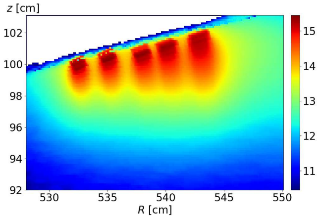
Figure 2. Synthetic image of the 706.5 nm line intensity in the poloidal plane at the gas nozzle location, medium plasma density case. Colorbar corresponds to \log_{10}(I[\text{photons/s/cm}^2/\text{rad}]) . The virtual camera is placed 1 m toroidally away from this plane and views perpendicularly onto it. T_e and n_e in the plane of emission are displayed in figure 3. Five beams, injected simultaneously at the upper divertor (interface between white and blue region), propagate downwards. Thermal spread in beam source, metastable states [13] and p-He elastic scattering [27] are included, no recombination. Beam parameters are taken from [6, 32]. Particle flux is \dot{N} = 1.5 \times 10^{19} \text{ s}^{-1} per beam.
