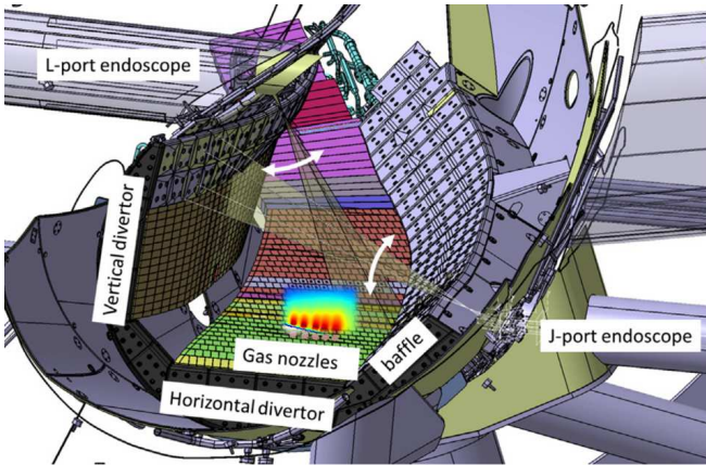
Figure 1. Gas inlets and observation geometry for spectroscopy in a lower W7-X divertor, amended from [17], plus simulated helium gas distribution (figure 2 mirrored vertically). The set-up in the upper divertor is equivalent up to vertical mirroring.
