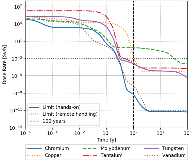
Figure 12: Activation Dose Rate
