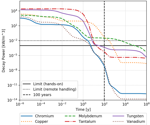
Figure 13: Activation Decay Power
