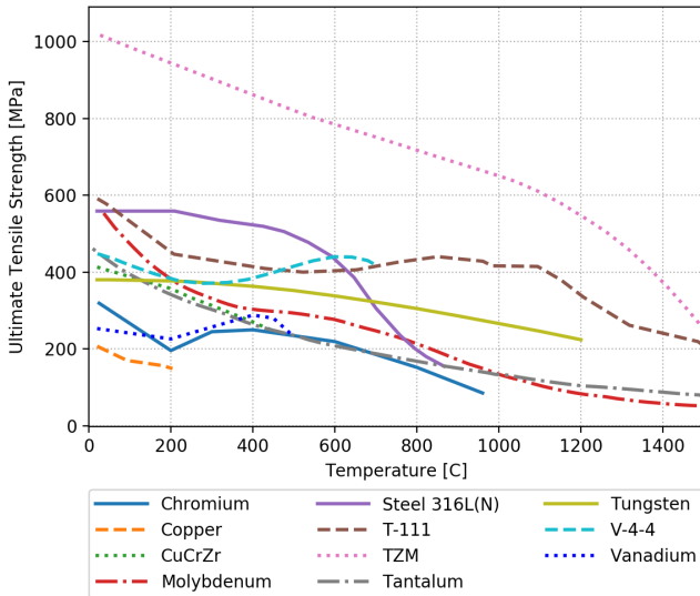
Figure 5: Ultimate tensile strength with temperature [32, 25, 34, 30]
