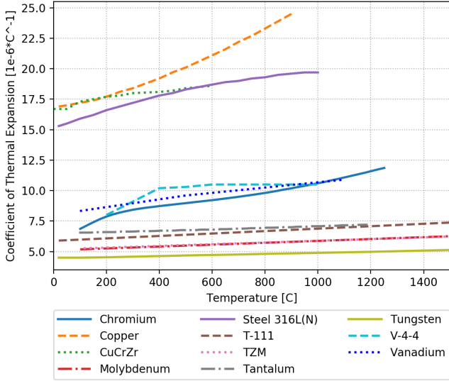
Figure 8: Thermal expansion with temperature [32, 25, 34, 30]
