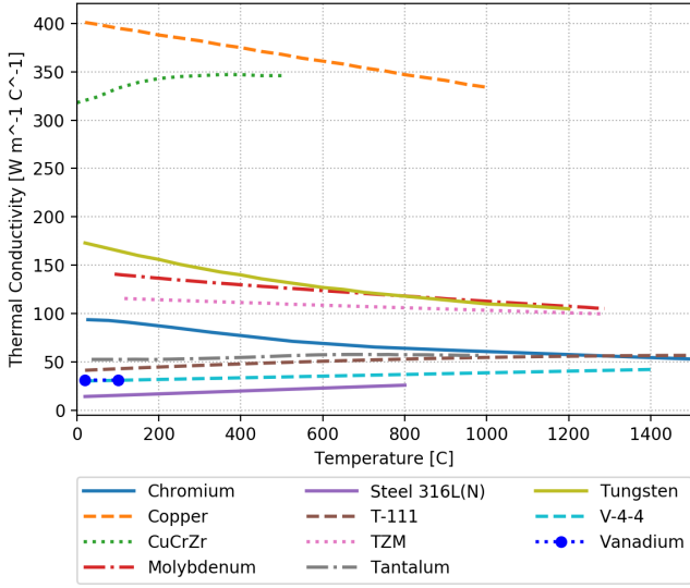
Figure 7: Thermal conductivity with temperature [32, 25, 34, 30]
