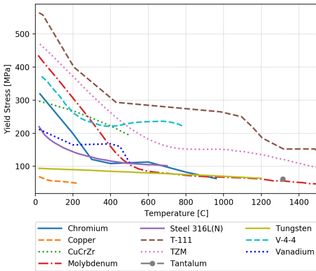
Figure 4: Yield stress with temperature [32, 25, 34, 28, 26]
