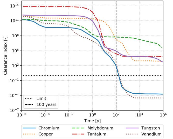
Figure 14: Activation Clearance Index
