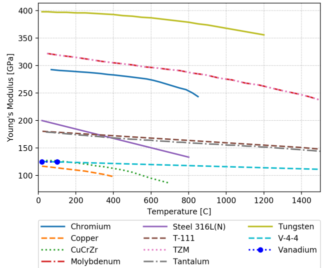
Figure 3: Young's modulus with temperature [32, 25, 34, 30]
