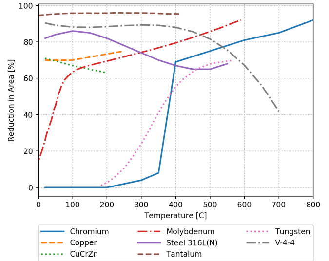
Figure 6: Percentage reduction in area with temperature [32, 26, 31]
