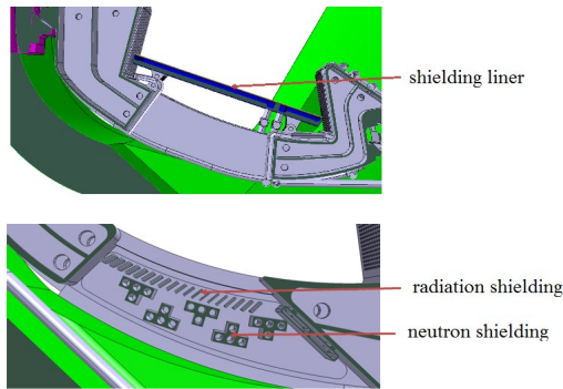
Fig. 5 Alternative solutions for vacuum pumping hole protection
