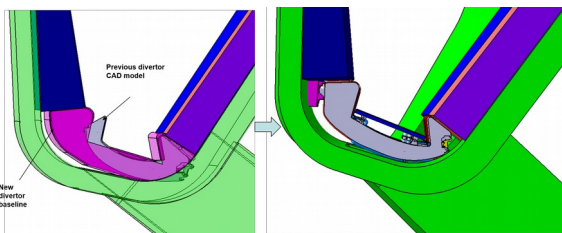
Fig. 1 (a) New baseline profile (in purple). (b) The 2017 divertor model – interface with VV and BB.
