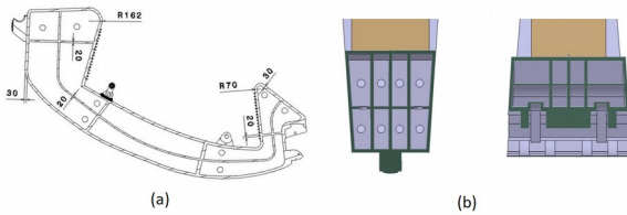
Fig. 3 (a) Divertor CB poloidal section, (b) Divertor CB toroidal section at inboard (left) and outboard (right)
