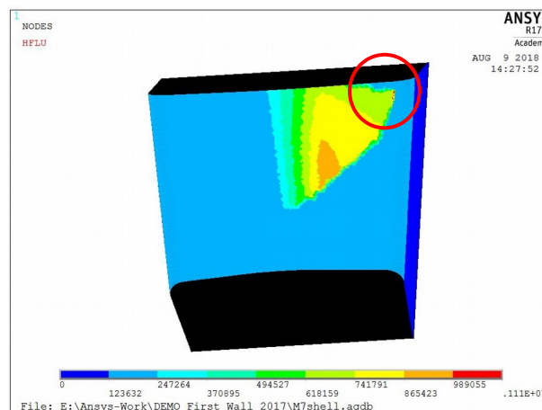
Figure 5: Imported heat flux on the ANSYS model (see Figure 2 to compare).
