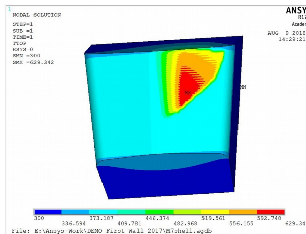
Figure 6: ANSYS result: Temperature distribution [°C] on module 7 surface (nominal case).
