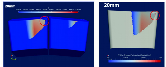
Figure 2: SMARDDA and PFCflux heat flux maps for module 7 with 20 mm normal translation (SOF)
