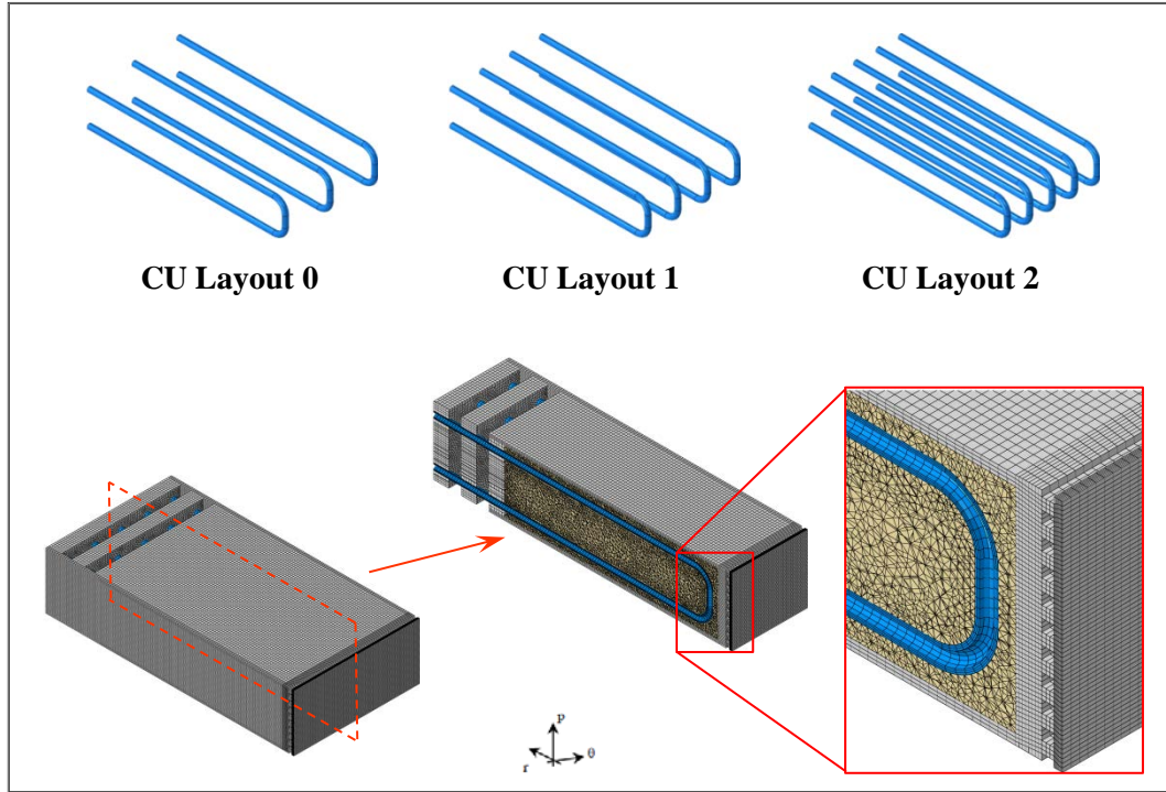
Fig.2. CU layouts and FEM models.
