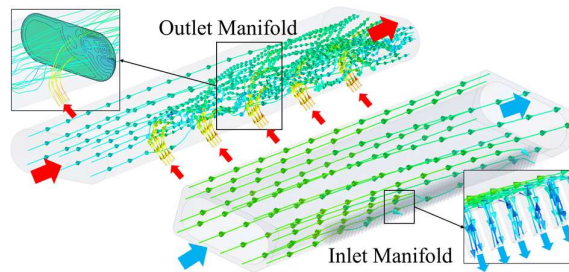
Fig. 3. 3D model of the BBS: computed streamlines in the Outlet (top) and Inlet (bottom) full-size manifolds. Details of the derivations are also shown.
