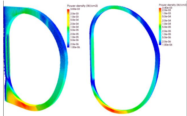
Fig. 4: Power density distribution in the TFC casing (left) and the super-conductor (right) of DEMO.
