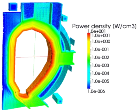
Fig. 3: Spatial distribution of the heating in a HCPB DEMO torus sector.
