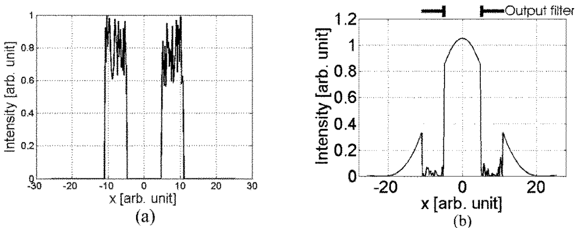
Figure 4. Output beam distribution (b) for a noisy (input) annular beam (a).
