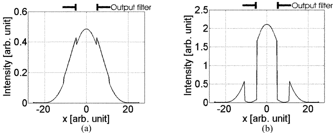
Figure 3. Output of the confocal telescope when the relative amplitude (a) and the phase (b) of the central lobe of the diffraction pattern are modulated (for details see text).
