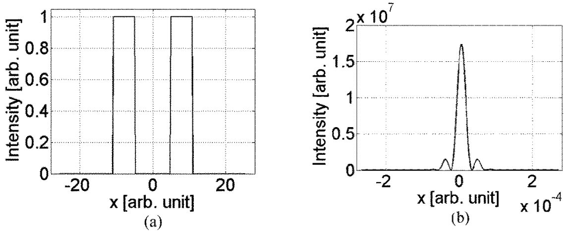
Figure 2. Cross-section of an annular beam (a) and its distribution in the focal plane (b).
