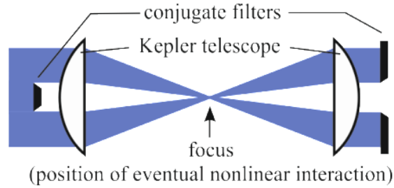
Figure 1. Schematic of the nonlinear filter.
