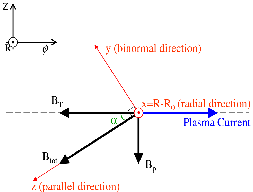
FIG. 5. Diagram of the coordinate systems used in the paper. In the upper left corner cylindrical system with radial, R , toroidal, \phi , and vertical, Z coordinates. The rest of the diagram shows how the cylindrical system is related to the field aligned coordinates used in the simulations: radial, x , bi-normal, y , and parallel, z . R_0 is a reference major radius, typically the position of first detection of the filament.
