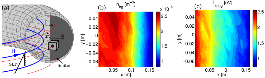
FIG. 1. (a) Schematic representation of the TORPEX experiment. The limiter located in the low-field side region is shown together with the probes used to perform blob conditional sampling. (b-c) Background profiles of n and T_e in the low-field side region, where blobs propagate. The profiles are measured in a poloidal plane 3 cm away from the limiter.
