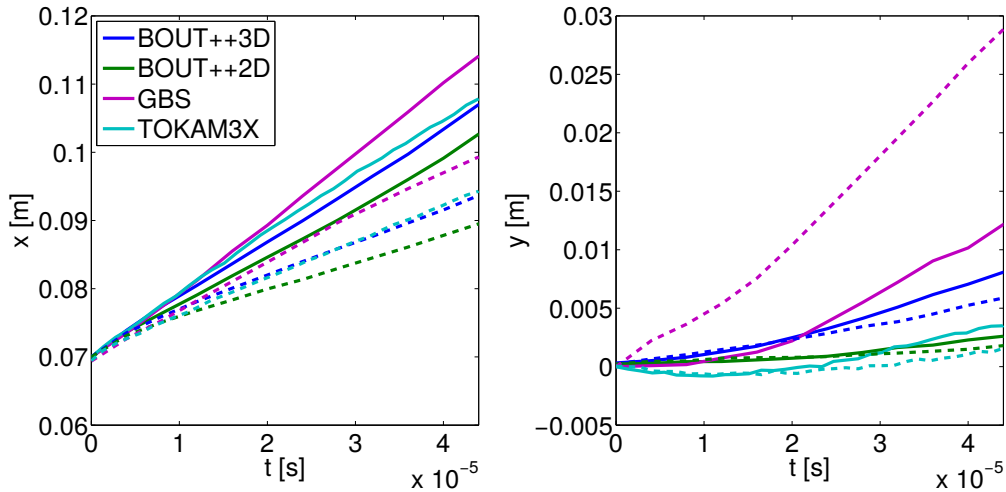
FIG. 4. Radial (left) and vertical (right) position of the blob as function of time for “case 1”. Solid curves represent the simulation results with T_{e,bg} = 2.8 eV, dashed curves consider T_{e,bg} = 1.85 eV for BOUT++3D, BOUT++2D, and TOKAM3X and T_{e,bg} given by Eq. (21) for GBS.
