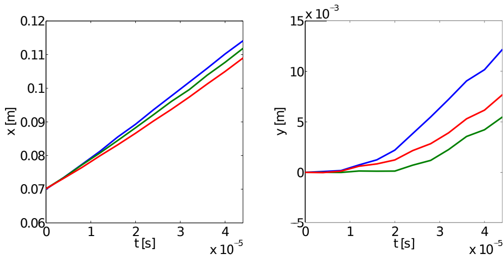
FIG. 5. Radial (left) and vertical (right) position of the blob as function of time, obtained from GBS simulations of “case 1” with T_{e,bg} = 2.8\text{ eV} . The blue curves correspond to an initially hot blob [i.e., T_{e,bl} = T_{e,bl}(x, y) at t = 0 , as in Eq. (24)], the green curves correspond to an initially thermalized blob (i.e., T_{e,bl} = 0 at t = 0 and then letting the blob temperature evolve), and the red curves correspond to an isothermal blob (i.e., imposing T_{e,bl} = 0 at all times).
