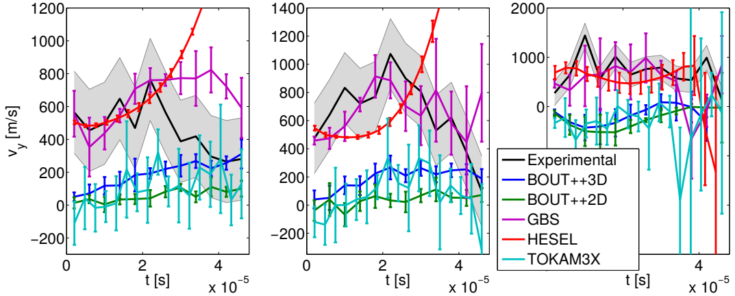
FIG. 8. Vertical velocity of the blob as function of time for “case 1” (left), “case 2” (middle), and “case 3” (right), obtained from numerical simulations and experimental measurements.
