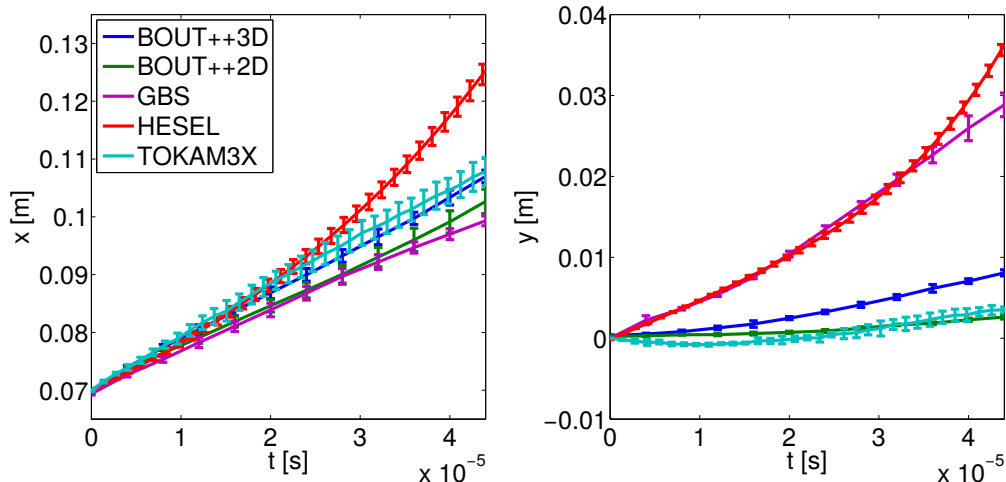
FIG. 3. Radial (left) and vertical (right) position of the blob as function of time for “case 1”, with errorbars representing the uncertainties affecting the numerical results due to the uncertainties on the initial conditions.
