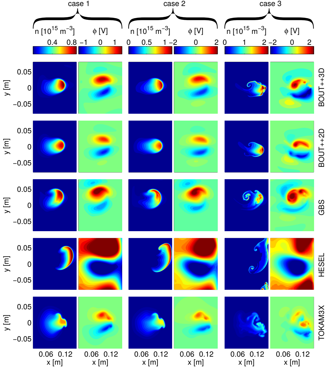
FIG. 6. Plasma density and electrostatic potential, for the “case 1”, “case 2”, and “case 3” blobs, simulated with BOUT++2D, BOUT++3D, GBS, HESEL, and TOKAM3X, at t = 48 \mu\text{s} . We note that for BOUT++2D and for HESEL the line averaged quantities n(x, y)/2 and \phi(x, y) are represented, while the profiles of n(x, y, z) and \phi(x, y, z) at the simulated poloidal plane closest to the limiter are displayed for the three-dimensional models.
