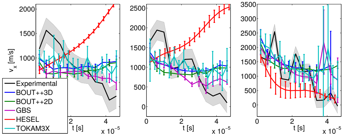
FIG. 7. Radial velocity of the blob as function of time for “case 1” (left), “case 2” (middle), and “case 3” (right), obtained from numerical simulations and experimental measurements.
