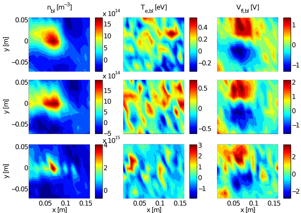
FIG. 2. Plasma density (first column), electron temperature (second column), and floating potential (third column) at detection time t = 0 , for “case 1” (first row), “case 2” (second row), and “case 3” (third row) conditionally averaged blobs, from which have been subtracted the backgrounds.
