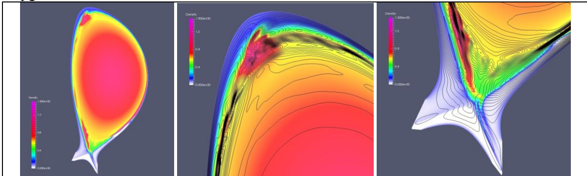
Figure 11. The density contour in colour and the potential contour in black lines during the pellet triggered ELM by 4.7mm pellet.
