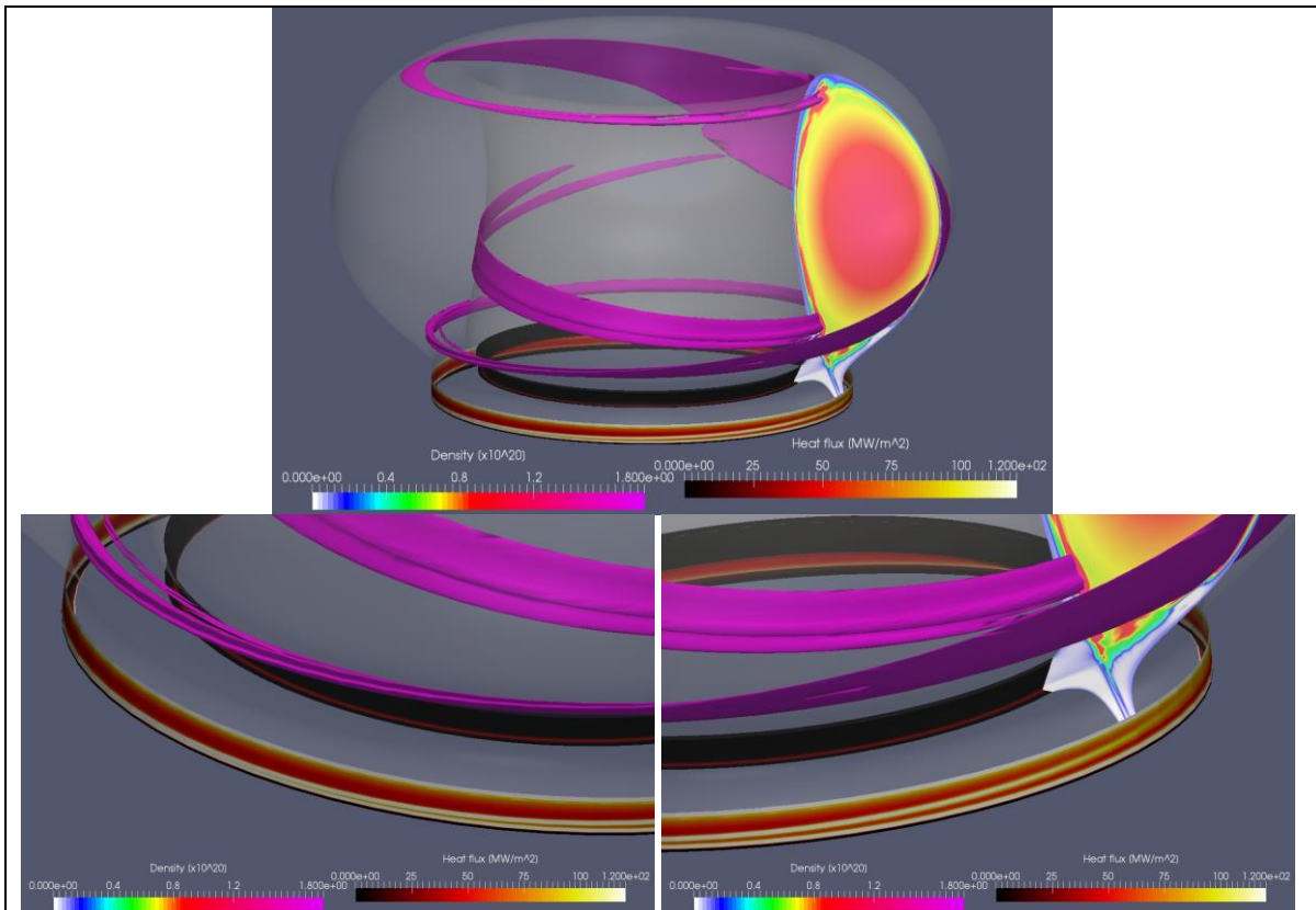
Figure 12. The profile of the heat flux on the outer divertor target by pellet injection of 4.7mm pellet. The toroidal asymmetry of the power deposition by pellet injection is observed.
