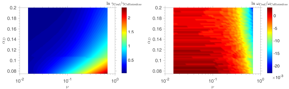
FIGURE 5. Damping rate \gamma (left) and oscillation frequency \omega (right) of the electron-plasma wave obtained from the moment-hierarchy equation, Eq. (2.16), as a function of \alpha_D and \nu for (P, J) = (18, 2) . The full linearized Coulomb collision operator is considered.
