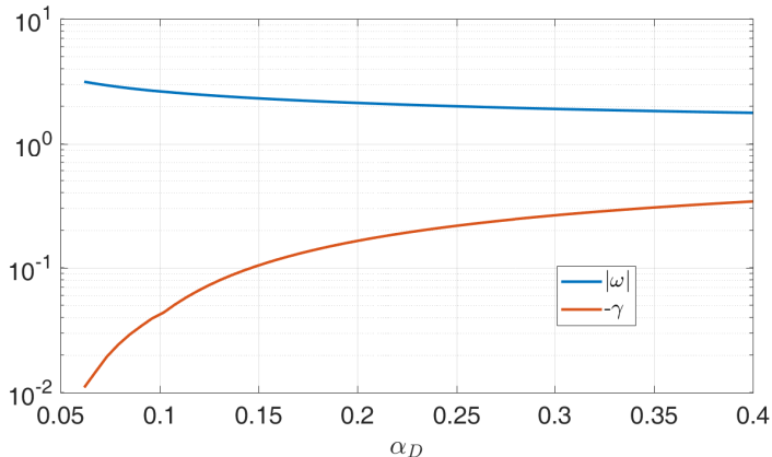
FIGURE 2. Collisionless frequency (blue line) and damping rate (red line) of the least damped solution of the collisionless dispersion relation, Eq. (3.4), as a function of \alpha_D , for 0.05 < \alpha_D < 0.4 .
