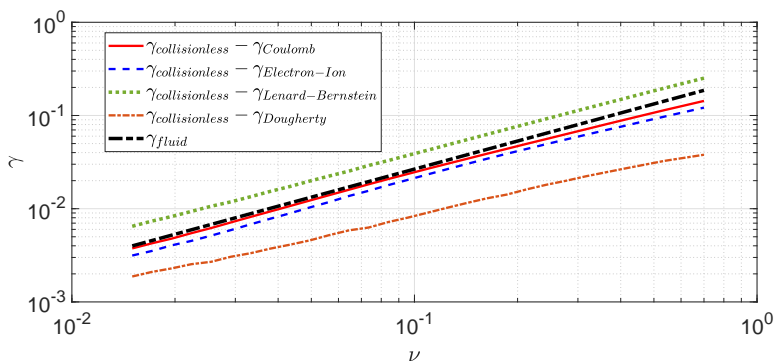
FIGURE 6. Difference between the collisionless damping rate \gamma with the one resulting from the moment-hierarchy equation, Eq. (2.16), with the full Coulomb, Lenard-Bernstein, Dougherty, and electron-ion collision operators at \alpha_D = 0.09 and (P, J) = (18, 2) . The collisional damping rate \gamma_{fluid} = -0.266\nu obtained from a fluid description is also shown for comparison.
