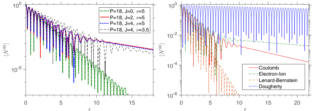
FIGURE 7. Time evolution of the absolute value of N^{00} with \nu = 5 and \alpha_D = 0.01 . Left: convergence study with a full-Coulomb operator and (P, J) = (18, 0) (green), (P, J) = (18, 2) (red), and (P, J) = (18, 4) (blue). The time evolution of N^{00} with \nu = 3.5 and (P, J) = (18, 4) is also shown for comparison (black). Right: truncation at (P, J) = (18, 2) using the full-Coulomb collision operator (red), electron-ion collisions only (green), the Lenard-Bernstein (orange) and the Dougherty (blue) collision operators.
