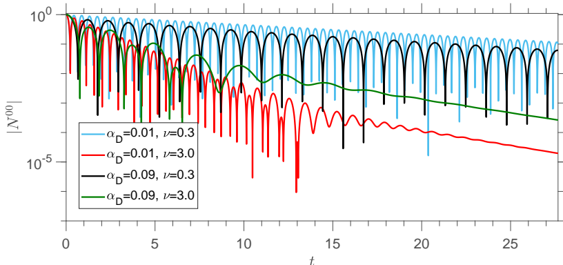
FIGURE 3. Time evolution of the absolute value of N^{00} using a truncation with (P, J) = (18, 2) , evaluated using the full linearized Coulomb collision operator. Different values of \nu and \alpha_D are shown.
