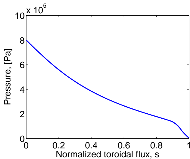
Figure 3: Pressure profile for a 15MA burning plasma in ITER plotted against normalized toroidal flux; high \vec{\nabla}p pedestal at s \approx 0.95
