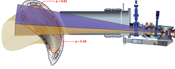
Figure 1: Viewing geometry of the the XICS diagnostic on W7-X.
