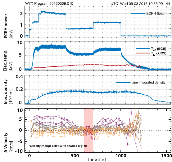
Figure 3: Time traces for W7-X CERC discharge. For clarity, the change in velocity seen in individual XICS sightlines is shown relative to the value at 650 ms. Purple and yellow lines represent views above and below the magnetic axis respectively (see Fig.1).
