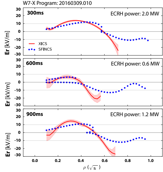
Figure 2: Radial electric field profiles ( E_r ) inferred from XICS velocity measurements. Spatial resolution is limited in the XICS measurements by strong smoothing during the inversion process. Also overlaid are calculated E_r profiles from the SFINCS neoclassical code.
