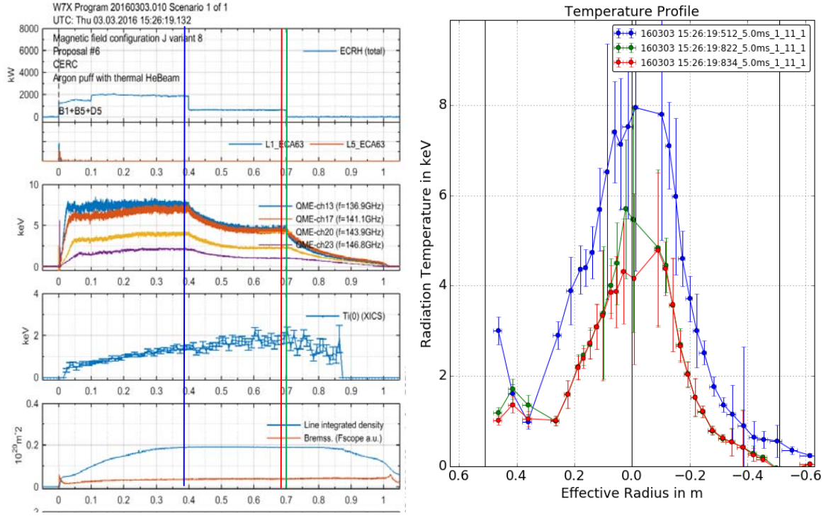
Fig.1: Left: Waveforms (from top to bottom) of ECRH heating power, selected ECE radiometer channels on the high field side, central T_i derived from X-ray imaging spectroscopy [5] and Bremsstrahlen (red) together with the line integrated density (blue) [6], for a discharge with power steps. Right: The ECE emission profiles shown, integrated over 5ms each, are selected at 390 ms (blue, 2 MW ECRH), 690ms (green, 0.8 MW ECRH) and 702ms (red, right after ECRH has been terminated).
