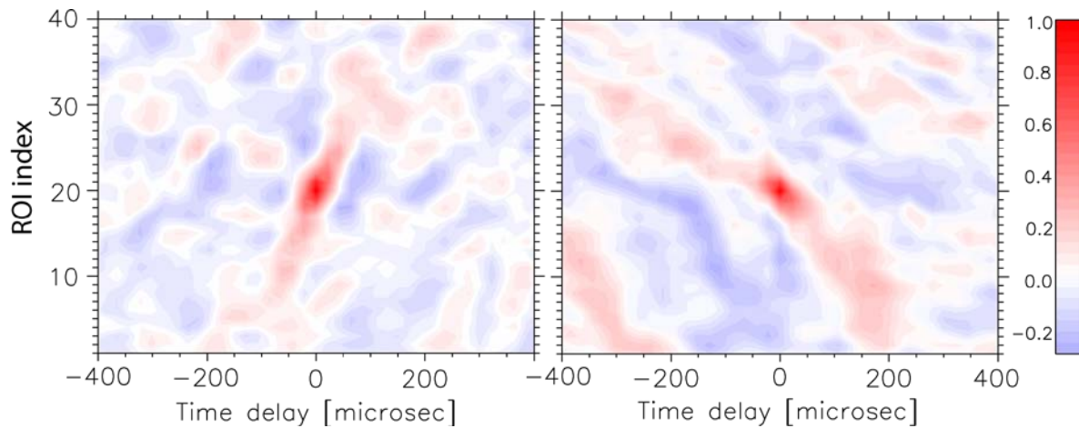
Fig. 3. Taking channel No. 20 as reference, the spatiotemporal correlation function of the surrounding channels as a function of the time lag for the above two time windows.
