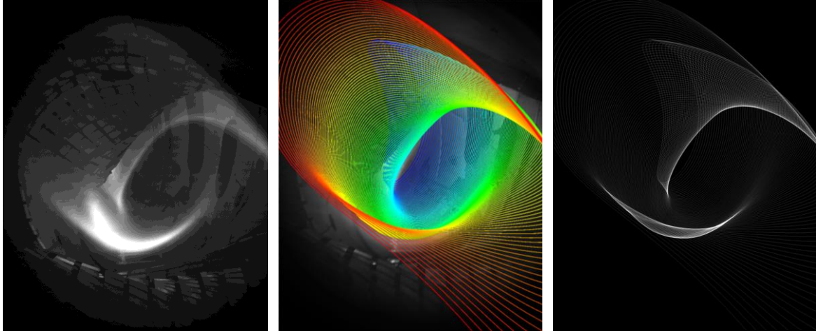
Fig.2. Left: EDICAM camera image. Middle: spatially calibrated image with LCFSs overplotted at several toroidal positions (denoted by colors: toroidal angle \varphi = 161-216^\circ red-blue). Right: synthetic image.
