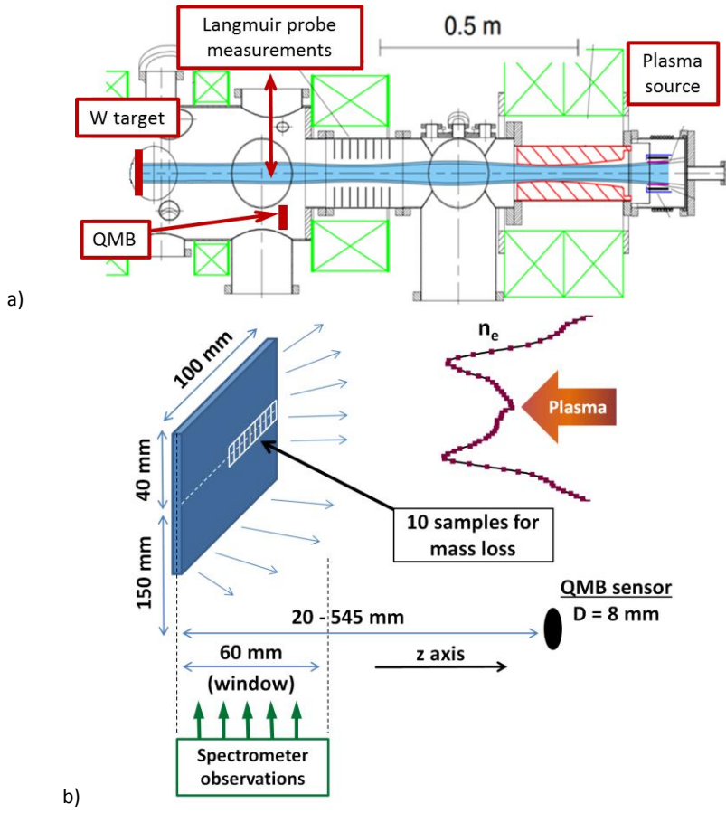
Fig.1. Scheme of the experimental set up on PSI-2: a) scheme of the installation with main diagnostics marked; b) scheme of the experiment with marked distances
