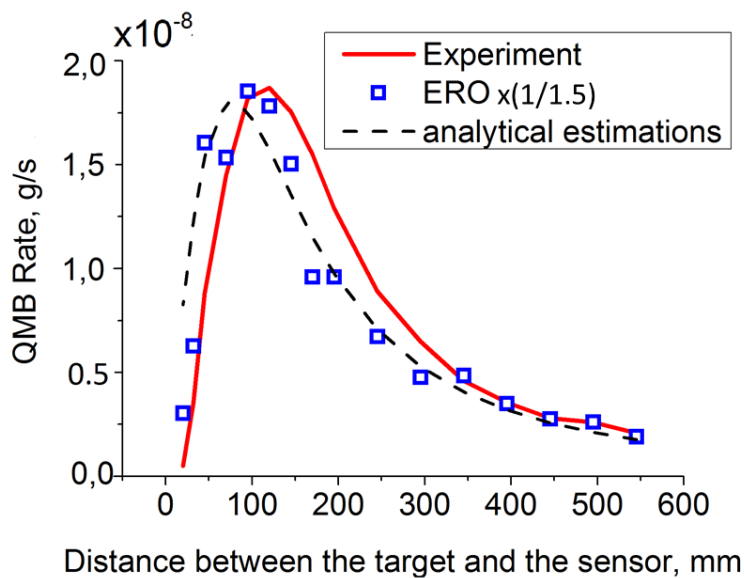
Fig.10. QMB rate as a function of the distance between the sensor and the target (Ar experiment, ERO simulation, analytical estimations based on geometry factors only)
