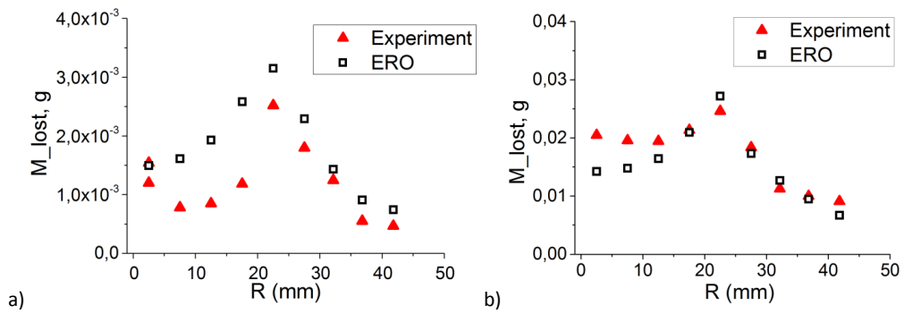
Fig.5. Weight loss values obtained from the Ar experiment and with the ERO simulations.
