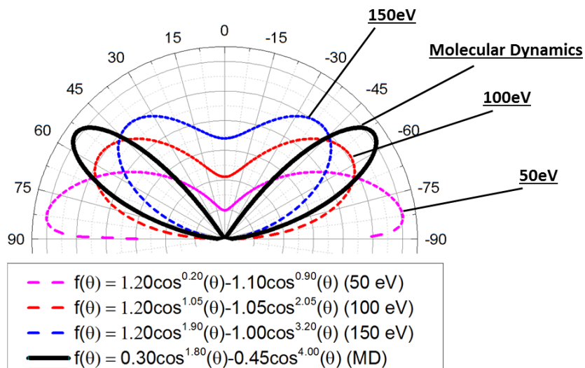
Fig.3. Angular distributions of sputtered W particles under Ar irradiation, approximated with (1). Dashed lines – approximation of experimentally obtained distributions from [19]. Solid line – approximation of PARCAS code MD simulations [20].
