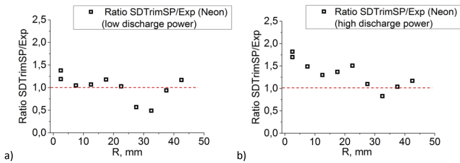
Fig.7. Ratio between SDTrimSp-calculated and experimentally obtained sputtering yields for Ne -> W experiments radial distribution.
