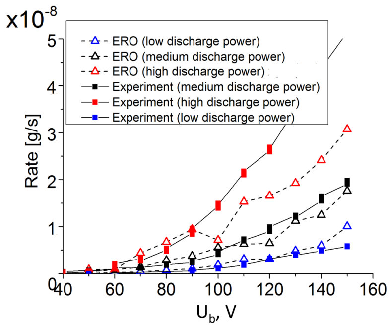
Fig.11. QMB rate as a function of bias voltage applied to the target ( U_b ) and discharge power (Ar experiment and ERO simulations)
