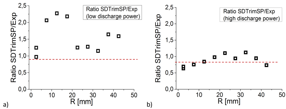
Fig.6. Ratio between SDTrimSp-calculated and experimentally obtained sputtering yields for Ar -> W experiments radial distribution. The redeposition of the impurities is counted out from the experimental yield based on the ERO calculations.
