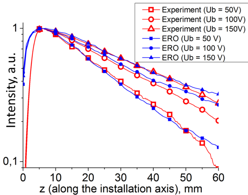
Fig.9. Axial WI ( \lambda = 400.9 \text{ nm} ) intensity profiles (normalized) – Ar experiment and ERO simulations. “Low” discharge power, U_b = 50\text{-}150 \text{ V} .
