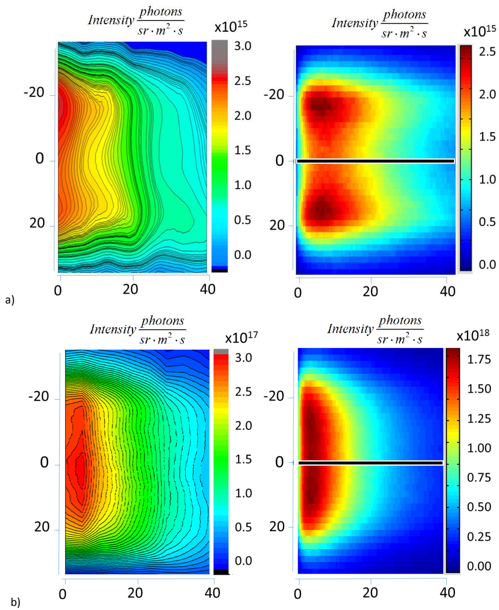
Fig.8. 2D sputtering patterns obtained in the Ar experiment with the spectrometer and calculated with ERO. Black line – direction of axial intensity profiles extraction.
