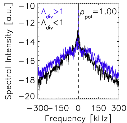
Figure 4: Power spectra of the complex amplitude obtained with F=41\text{GHz} in inter-ELM H-mode plasmas.
