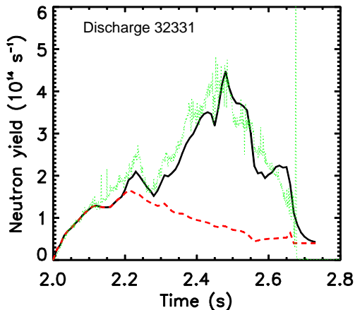
Figure 2 Measured (green) and simulated (black) R_{NT} as given by PION for discharge 32331. The measured R_{NT} has been scaled to match the simulated R_{NT} at t = 2.25 s. Also shown is R_{NT} as calculated by PION assuming zero ICRF power (red dashed line).
