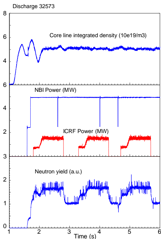
Figure 4 Overview of discharge 32573. The neutron yield is measured by an epithermal neutron detector.
