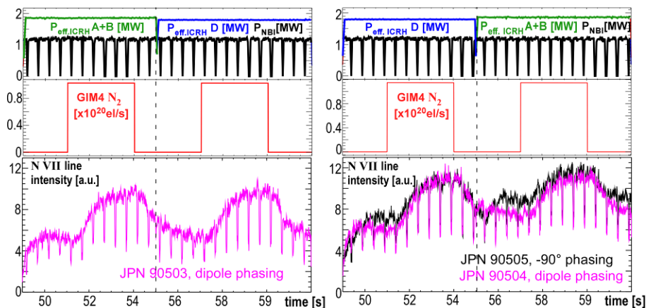
Fig. 6. Reaction of the core nitrogen content (N VII spectral line) during pulsed injection of nitrogen close to antenna A. Left: dipole phasing. Right: antenna order swapped, dipole and -90^\circ strap phasing.
