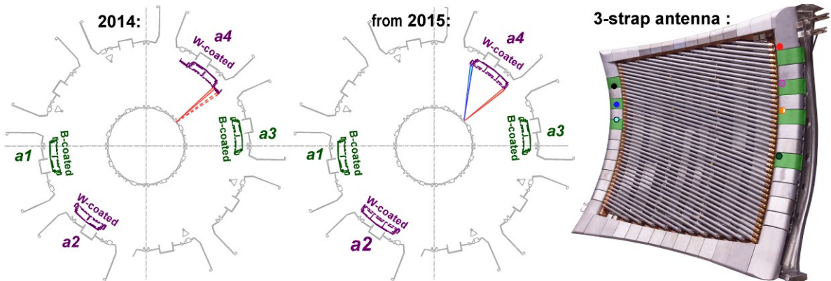
Fig. 1. Left: 2014 AUG antenna configuration. Middle: configuration from 2015. Right: view of AUG 3-strap antenna a4 and diagnostics.
