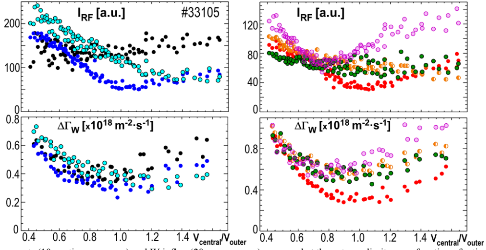
Fig. 4. RF currents (10 ms time averages) and W influx (20 ms averages) measured at the antenna limiter as a function of ratio of voltages at the feeders. Left: left side of a4 as seen from plasma, right: right side of a4 . Symbol code is the same as indicated on the limiter tiles in Fig. 1, right side.
