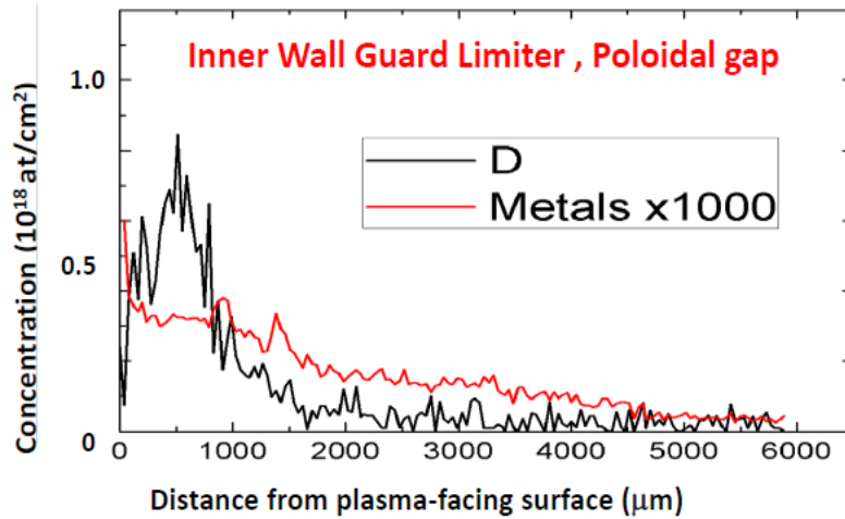
FIG. 3. Deposition profiles of deuterium and metals inside the castellated groove of a beryllium limiter.
