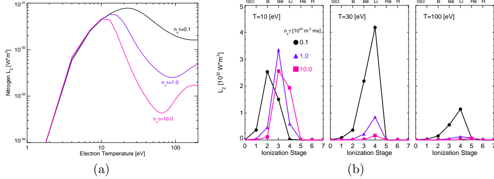
Figure 2: (a) Demonstration of the enhancement of nitrogen radiation for ions out of ionization equilibrium, showing a large increase in L_Z as n_e \tau is reduced and (b) how this enhanced radiation is distributed among different ionization stages.
