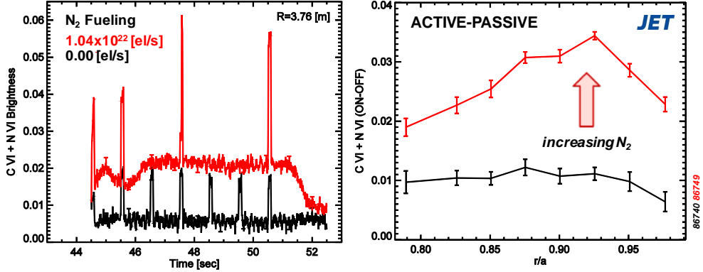
Figure 6: Demonstration of active and passive N VI charge exchange showing enhancement during NBI (left) and the transition from C VI dominated to mixed N VI and C VI emission profile (right).
