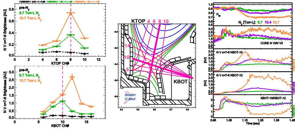
Figure 8: Example of spectroscopic methods implemented at Alcator C-Mod where spatial profiles of N V n=7-6 emission in the divertor are tracked as private flux nitrogen fueling is increased shot-to-shot. Movement of emission layers is shown to follow confinement degradation.
