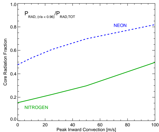
Figure 4: Resulting change in spatial structure of the 1D radiation profile computed from STRAHL simulations, showing an inward shift of radiation as convection is decreased to -100 m/s.
