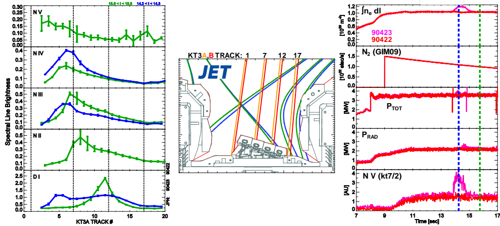
Figure 7: Example of enhanced spectroscopic tools used in JET L-mode experiments. Spatial profiles of D I and N II-V (left) are shown for chords viewing across the outer divertor (middle) at two different time points in repeated discharges that employed a weak strike point scan (right).
