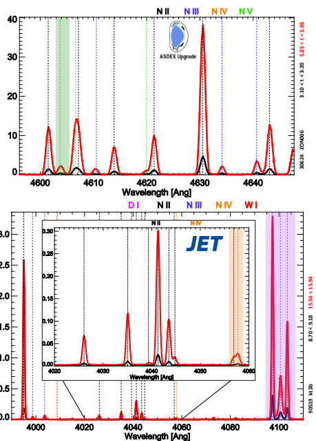
Figure 5: Measured spectra from boundary plasma showing ranges to observe N V (top) and N II-IV (bottom). High resolution is required to avoid overlap with D I and N II lines for N III, N IV and N V.
