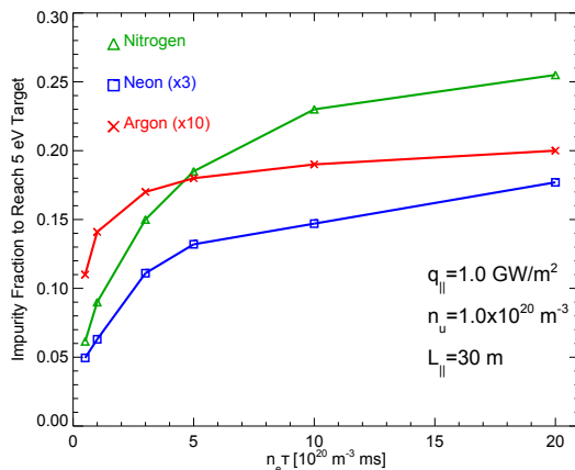
Figure 1: Estimation of impurity fraction necessary to reduce the temperature of a flux tube with given q_{\parallel} , n_u and L_{\parallel} as n_e \tau is varied.
