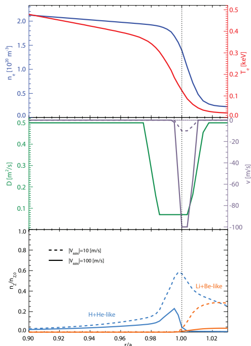
Figure 3: (top) STRAHL input T_e and n_e profiles with (middle) diffusion and convection profiles estimated to model an edge transport barrier. A limited range of charge state density profiles (bottom) are plotted for two possible peak convection values.
