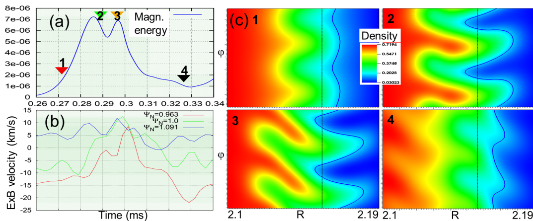
FIG. 2: (a) Magnetic energy of the n = 8 mode. (b) E \times B velocity inside pedestal (red), on separatrix (green) and in the SOL (blue). (c) Density filaments for the times given in (a).
