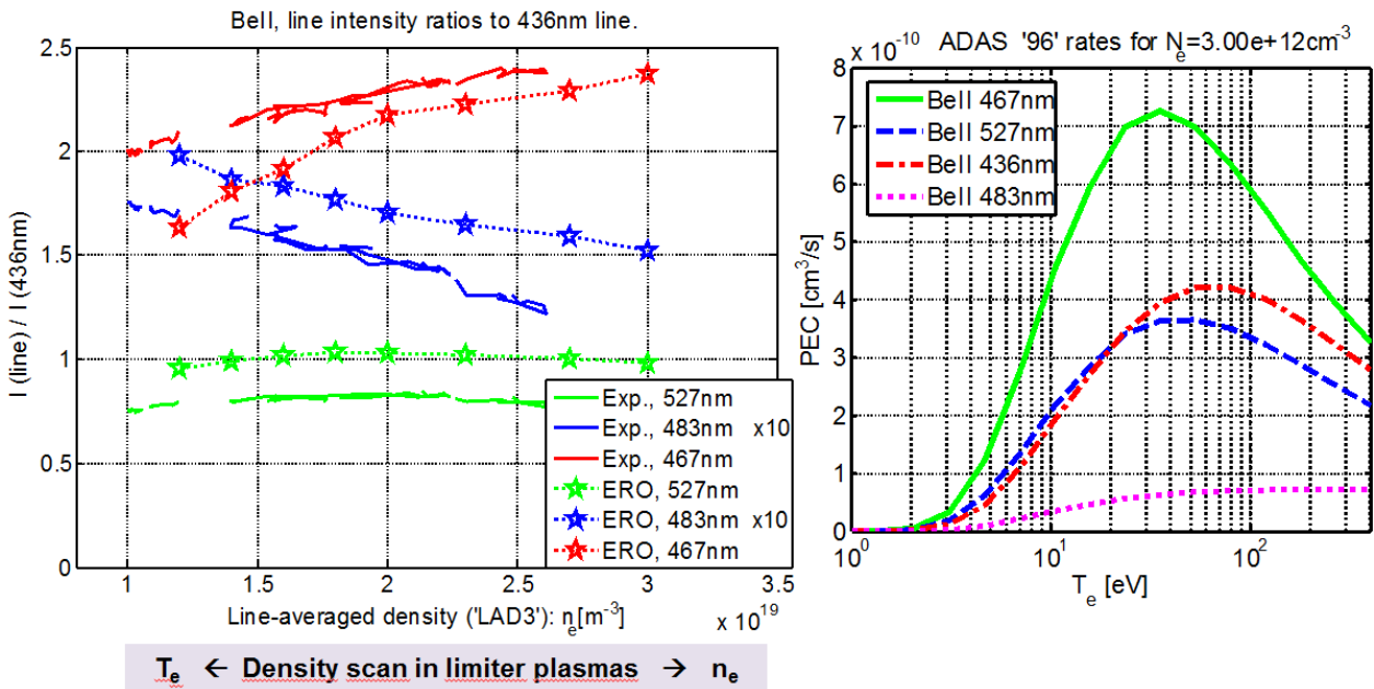
Fig. 4. Line ratios in BeII sputtered from the IW GL (left) and the relevant photon efficient coefficients from ADAS (right) [14].
