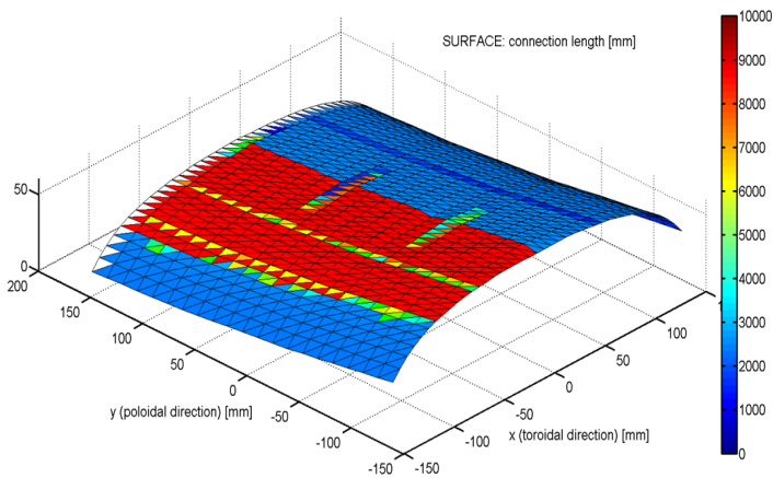
Fig. 1. The connection lengths simulated by the PFCFlux code [12] along the IWGL limiter surface part (3 tiles) included into the ERO simulation volume.
