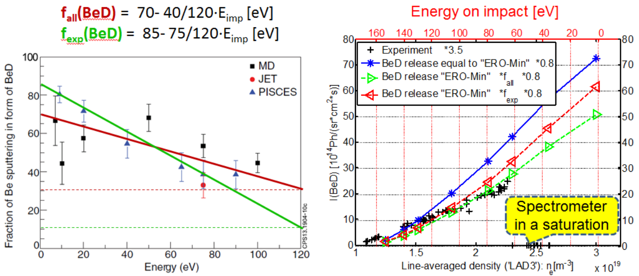
Fig.8. The BeD band emission simulated by ERO (total) and observed in experiment (right) using the fits for the fraction of BeD release from obtained on the experimental ('PISCES', 'JET') and simulated ('MD') data from [5]. Measurements are multiplied by 3.5 to obtain the total band intensity whereas only a fraction is coming into the spectral window.
