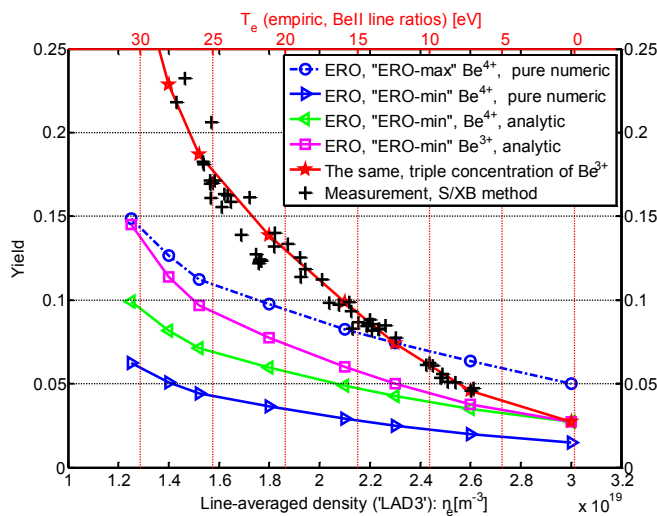
Fig. 6. The effective sputtering yields in ERO and S/XB method measurements. The influence of the physical sputtering fits for pure Be ('ERO-max') and Be with 50%D in the interaction layer ('ERO-min') [3]. The influence of the recently implemented analytical expressions [10] is shown ('analytic') as well as influence of the intrinsic Be impurity concentration and respective self-sputtering.
