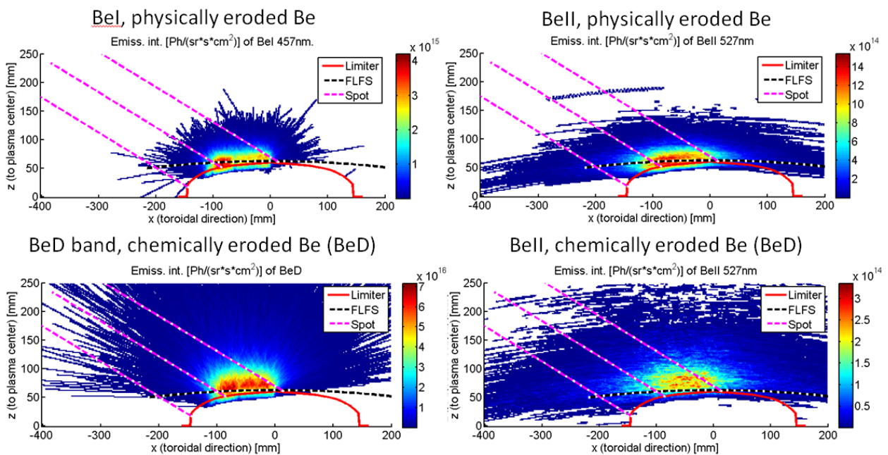
Fig. 2. BeI and BeII light emission in the close to the solid Be shaped IW limiter. ERO simulations for Be sputtered from the wall physically alongside with the simulations for chemically released BeD. BeII plume is determined by the shadowing local transport and ionization/dissociation.
