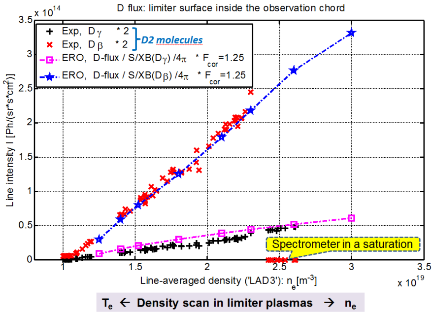
Fig. 3. D spectroscopy (Balmer- \alpha and Balmer- \beta ) characterizing the plasma ion flux to the surface. Experimental results are multiplied by 2 to account for the mostly molecular D release as D 2 which dissociates preferably through the channel with ionization of one of the atoms; this way every second released D atom is lost for the observation.
