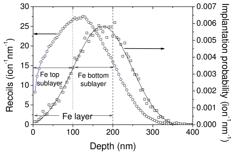
Fig.1. Recoils and implantation profile for 490 keV Fe + on Fe target according to SRIM calculations. For the definition of top and bottom Fe sublayer refer to Fig. 8a.
