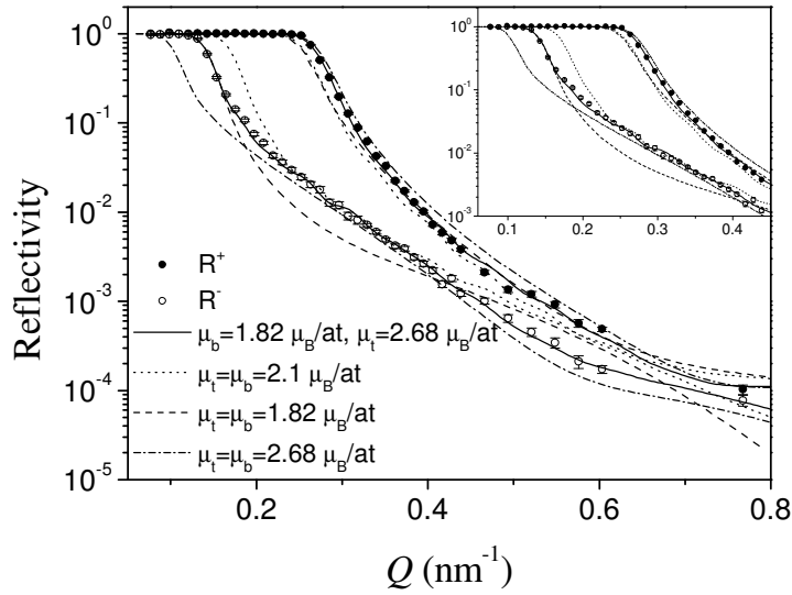
Fig.7. PNR data of sample irradiated at 96.2 dpa. The solid line is a least-square fit to the data with \mu_b=1.82 \mu_B/\text{at} and \mu_t=2.68 \mu_B/\text{at} . The dotted, dashed and dashed-dotted lines correspond to models with \mu_b= \mu_t=2.1 \mu_B/\text{at} , \mu_b= \mu_t=1.82 \mu_B/\text{at} and \mu_b= \mu_t=2.68 \mu_B/\text{at} , respectively (see 3.2 for further explanation). The inset shows the spin up and down reflectivity near the critical region.
