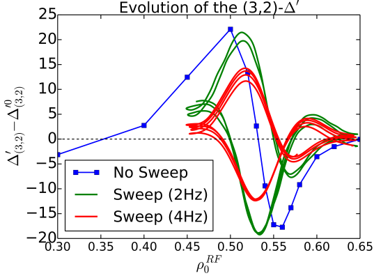
Figure 3: Effect of ECCD on \Delta'_{(3,2)} .
