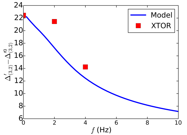
Figure 5: Variation of the maximum reached \Delta'_{(3,2)} for different frequencies of the sweeping.
