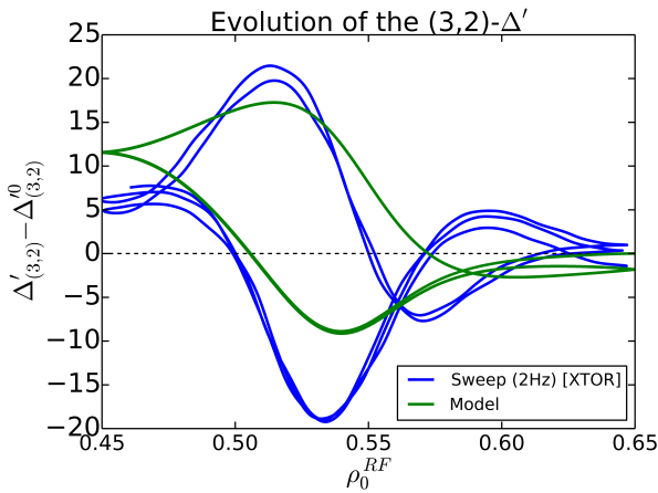
Figure 4: Evolution of \Delta'_{(3,2)} procuded by the analytical model (equation 1) and XTOR.
