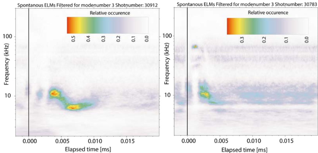
Fig. 3. Time-frequency mode number analysis for toroidal mode number 3 for the non-seeded and seeded scenario.
