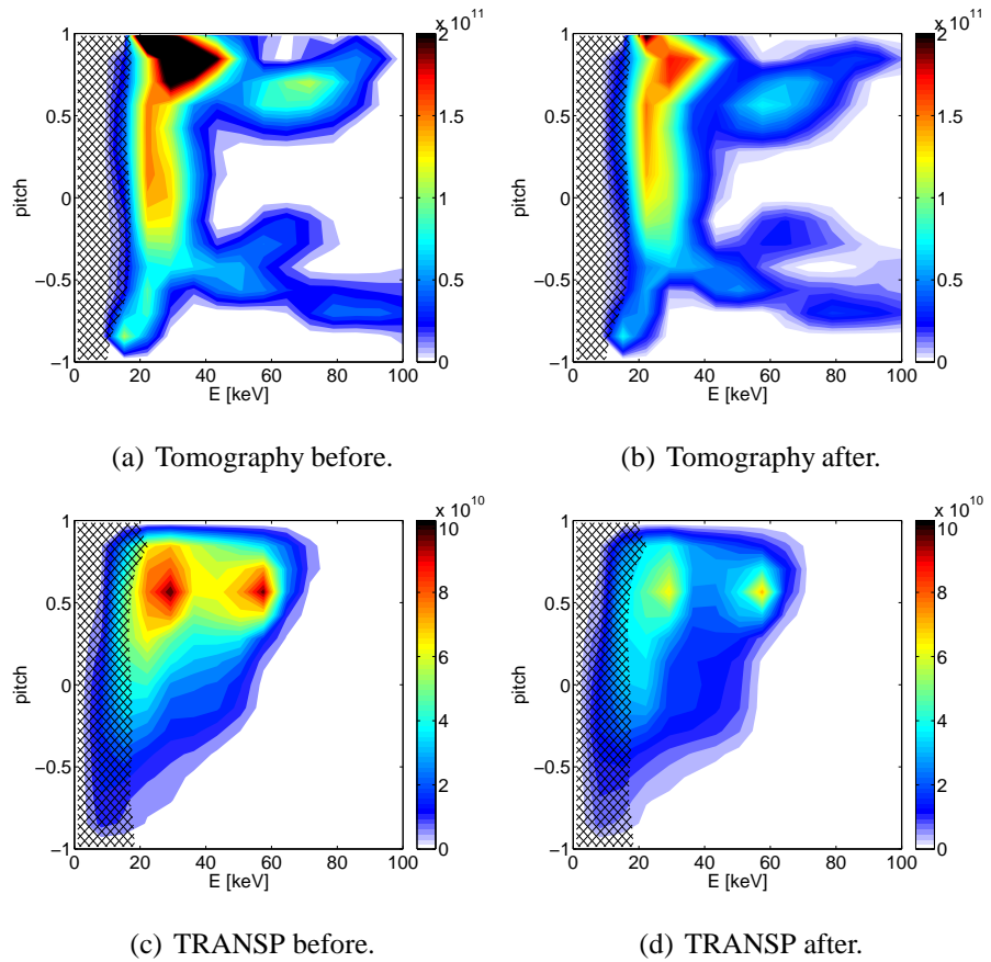
Figure 1: Central fast-ion velocity distribution functions before and after a sawtooth crash in units of [\text{ions/keV/cm}^3] .
