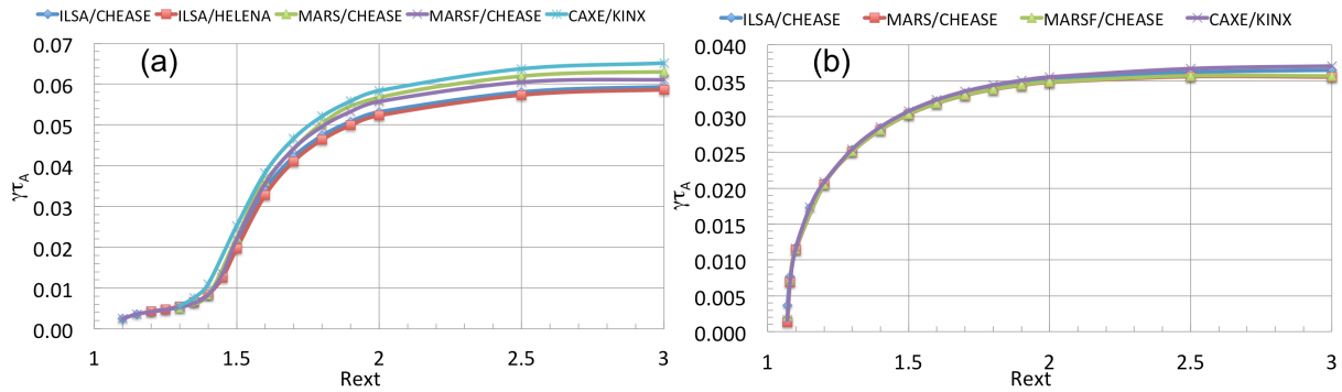
Figure 3 – Growth rate scaling of n=1 mode with wall position for JET (a) and AUG (b) equilibrium
