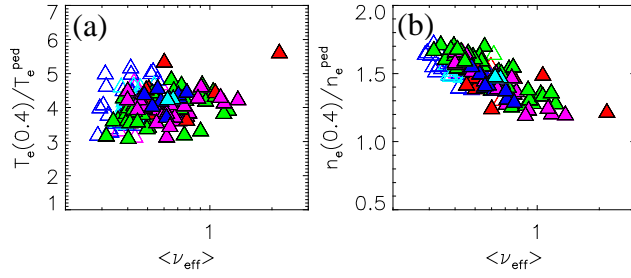
Figure 4. (a) T_e peaking vs \nu_{eff} ; (b) n_e peaking as a function of \nu_{eff} . Open symbols – JET-C, full symbols – JET-ILW. Colors correspond to levels of I_p .
