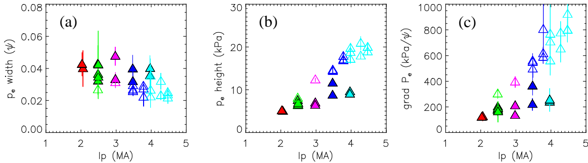
Figure 5. (a) p_e pedestal widths vs I_p ; (b) p_e pedestal heights vs I_p ; (c) grad p_e vs I_p . Open symbols – JET-C, full symbols – JET-ILW.
