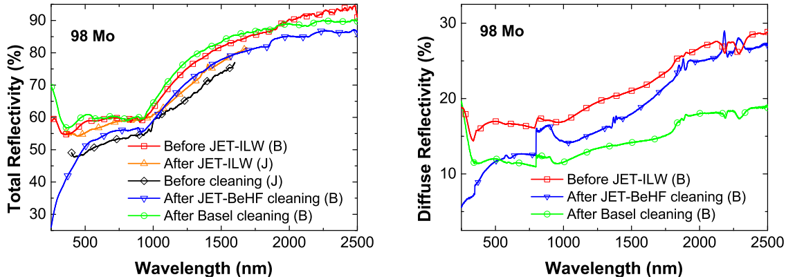
Figure 4: Total and diffuse reflectivity measured in JET (J) and/or Basel (B) before exposure in JET-ILW (denoted before JET-ILW), before and after cleaning in the JET-BeHF and after additional cleaning in Basel.
