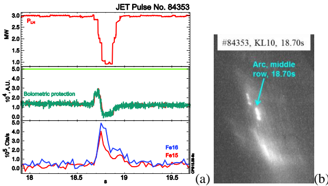
FIGURE 4. (a) Time traces of PLH, radiation protection signal and Fe15, Fe16; (b) arc as seen on KL10 camera in the middle of the grill. Arc has been quickly quenched in time to prevent large influx of Fe and disruption.
