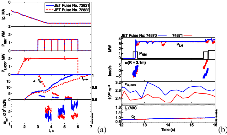
FIGURE 2. (a) Time traces of I_p , P_{NBI} , P_{LH} , q_0 , I_i and \omega_{tor}(R_0=3.05m) in LH (red) and non-LH (blue) preheat JET pulses; (b) time traces of P_{NBI} , P_{LH} , \omega_{tor}(R_0=3.1m) , n_e , I_p and q_0 for a pulse with the typical core-counter rotation (blue) and an exception with core co-rotation (red).
