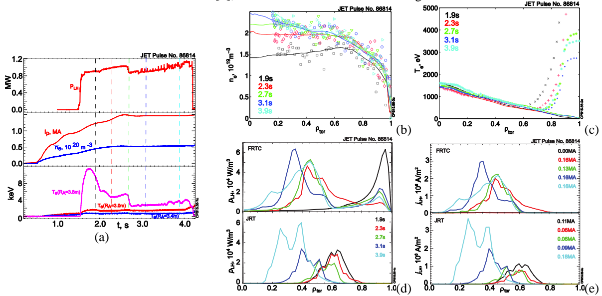
FIGURE 3. (a) Time traces of AT scenario pulse #86814, 2.4T/1.5MA, with n_e and T_e profiles at five time slices in (b) and (c); (d) Power deposition profiles from the new code JRT compared to FRTC at the five time intervals; (e) LH current drive for JRT and FRTC. The total driven current at each time slice is provided for comparison.
