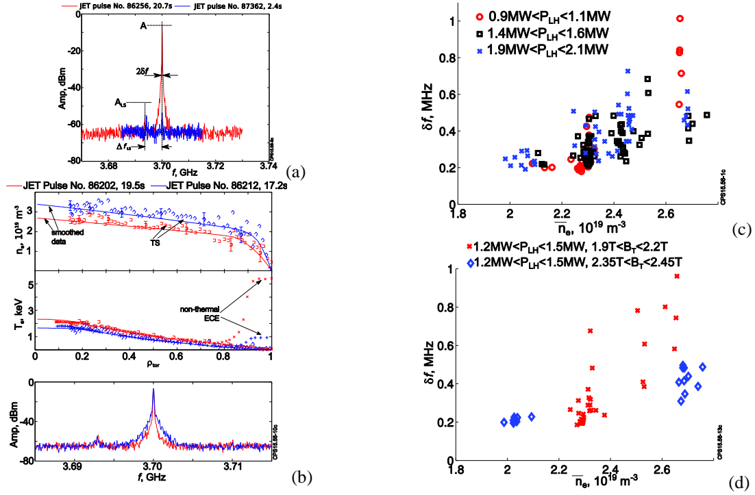
FIGURE 1. (a) RF spectra from reflected power data (#86256, 20.7s, in red) and RF probe (#87362, 2.4s, in blue); (b) Comparison between low (#86202, 2.37T/1.8MA, in red) and high density (#86212, 2.42T/1.8MA, in blue) JET pulses. The RF spectra are in the bottom graph. Density and electron temperature from Thomson Scattering (TS) are indicated with squares and diamonds, Electron Cyclotron Emission (ECE) temperature is shown in ‘x’ and ‘+’ and the solid lines are the smoothed profiles; (c) RF spectra broadening, \delta f , versus line averaged density, \bar{n}_e for low (red circles), intermediate (black squares) and high (blue crosses) P_{\text{LH}} ; (d) RF spectra broadening, \delta f , versus \bar{n}_e for low (red x) and high (blue diamonds) B_{\text{T}} . P_{\text{LH}} is between 1.2 and 1.5MW. All data in (b), (c) and (d) were taken from reflected power measurements.
