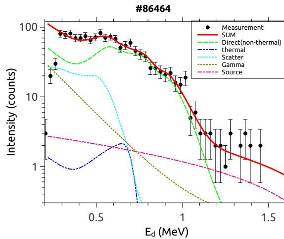
Figure 4: SDD spectrum measured at JET for discharge #86464 with radio-frequency heating at the third harmonic applied to an injected beam of deuterium. A fit of the spectrum using the same analysis procedure as for figure 2 is superimposed to the data
