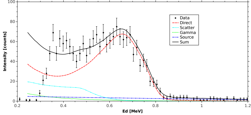
Figure 2: SDD spectrum measured at JET for discharge #84476 with neutral beam injection, as a function of the deposited energy E_d . A fit to the data is also shown. The components considered in the data analysis are direct neutrons from the plasma (direct), scattered neutrons (scatter) and background gamma-rays (gammas), as well as the background arising from the \alpha calibration source (source).
