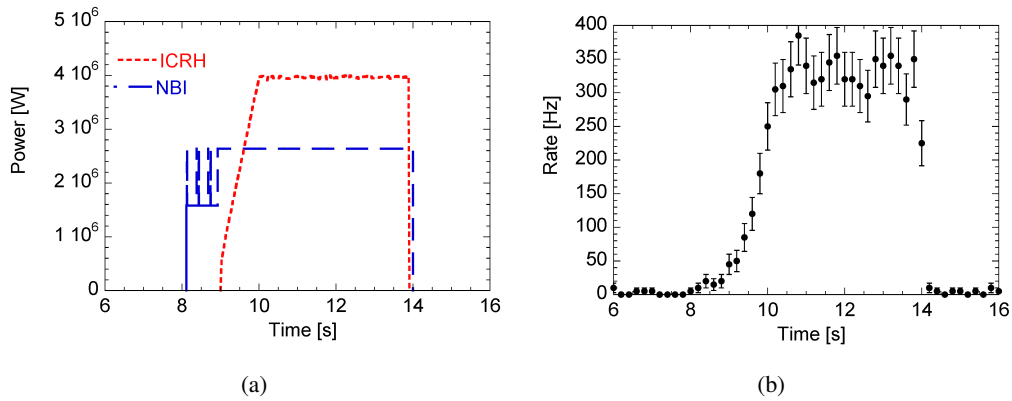
Figure 3: a) Time trace of the auxiliary heating used in discharge #86464 with radio-frequency heating at the third harmonic on an injected beam of deuterium. b) Counting rate as a function of time measured by the SDD during the auxiliary heating phase.
