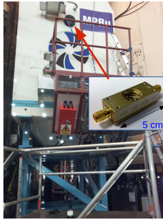
Figure 1: Photograph of the SDD installed at JET in the MPRu beam dump
