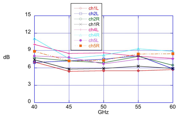
Figure 3: Measured losses after installation in the octant of the transmission lines of the two antenna (called Left (L) and Right (R)) for some of the different reflectometer's channels
