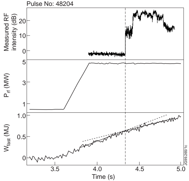
Fig.4: Upper: plot of the MICE intensity at 29.6 MHz. The noise floor is at 0 dB. Middle: trace of the ICRH power coupled to the plasma at 37.3 MHz. Lower: plot of the total anisotropic component of the plasma stored energy ( W_{fast} ), associated with ICRH minority ions.
