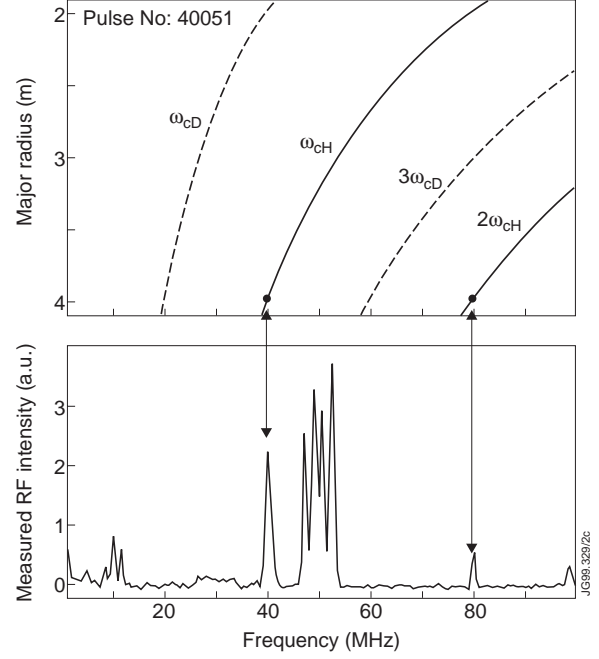
Fig.3: Lower: rf emission spectra measured during four-frequency ICRH. Fundamental and second harmonic MICE lines are visible at 40 MHz and 80 MHz in this discharge.
