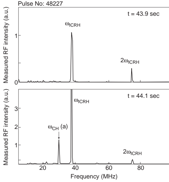
Fig.2: Rf emission spectra measured during single-frequency ICRH. Upper: spectrum measured 240 ms after ICRH flat-top reached; lower: spectrum was measured 440 ms after ICRH flat-top reached and showing the MICE line at 29.6 MHz.
