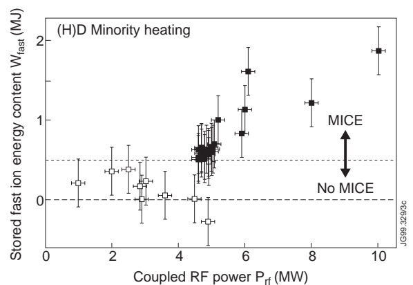
Fig.5: Existence diagram for MICE constructed from a database of discharges with (H)D ICRF heating displayed in the ( W_{fast} , P_{rf} ) plane. Filled symbols denote MICE detected; open symbols denote MICE not detected.
