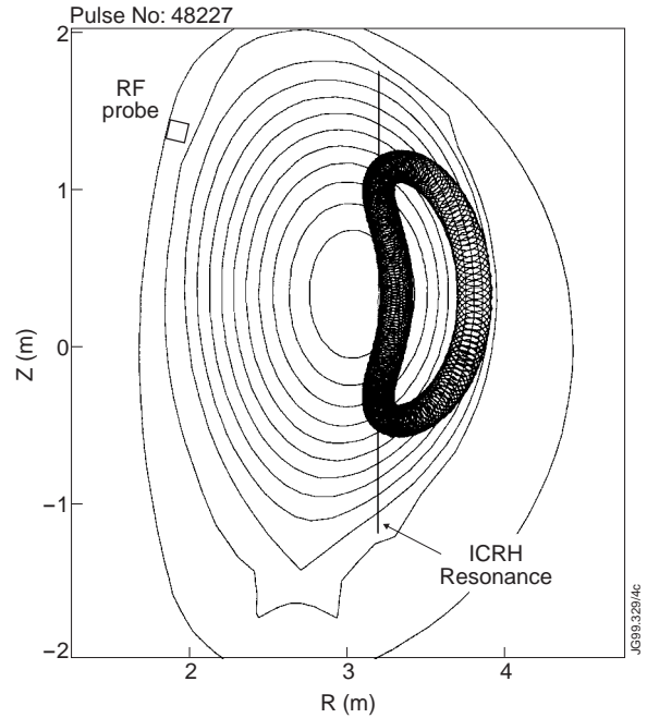
Fig.1: Poloidal cross-section geometry of the JET tokamak showing the flux contours of a typical X-point discharge (shot 48227 at time 4 s) with ICRH. The diagnostic rf probe antenna is shown as well as the D-shaped orbit of an ICRH 3 MeV minority proton.
