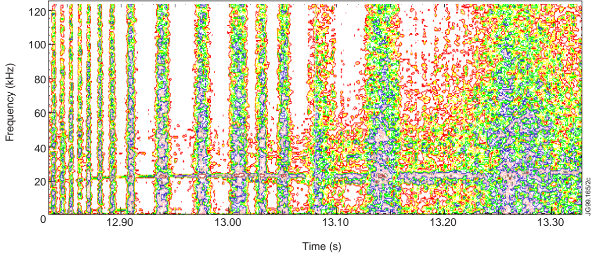
Fig.2: Contour plot of log spectral intensity (frequency vs time) of phase fluctuations signals shown in Fig.1 (shot #40477). Note coherent mode at 20kHz.
