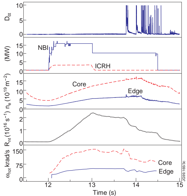
Fig.3: Plasma parameter time traces for ELM-free Hot-ion H-mode shot #40477.
