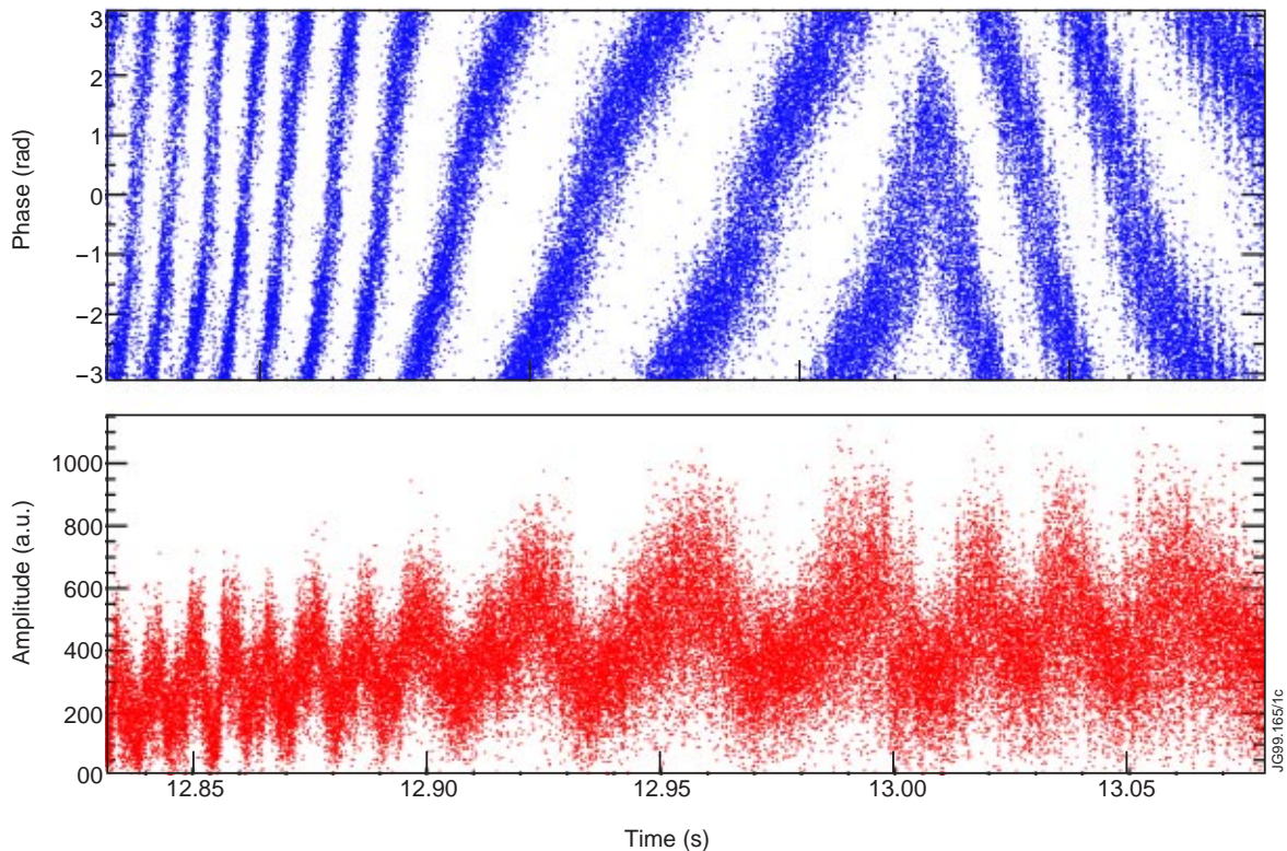
Fig.1: 250ms long time traces of raw phase and amplitude signals from a 105GHz X-mode reflectometer ( r/a \sim 0.8 ) during JET shot #40477. Sample period is 4\mu\text{s} .
