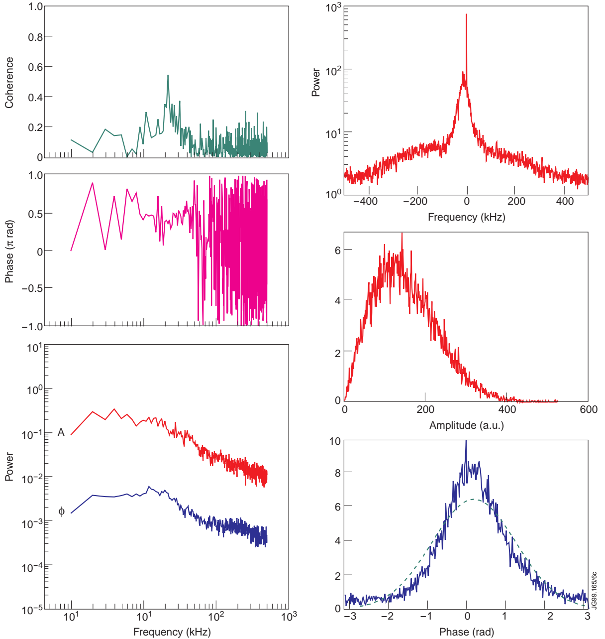
Fig.6: Fourier, coherence and cross-phase spectra, with phase and amplitude pdf, and double-sided complex amplitude spectra of experimental signals shown in Fig.5.
