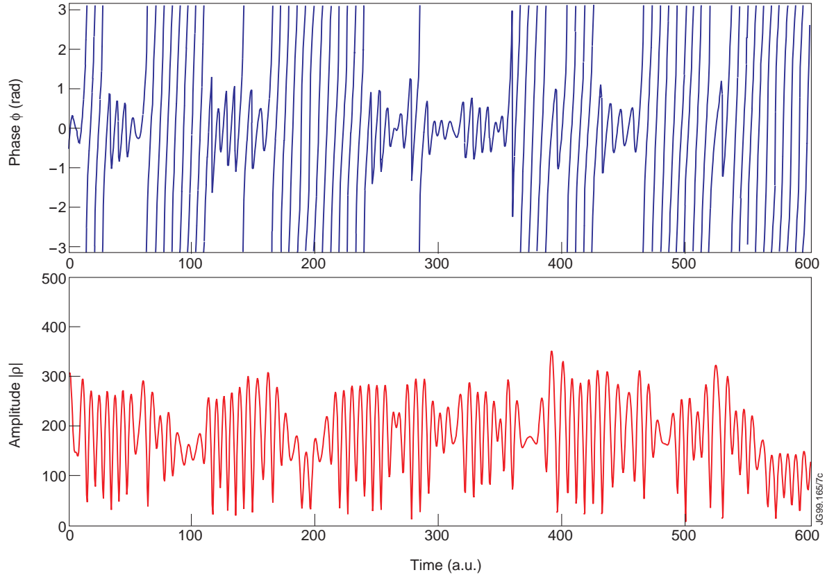
Fig.7: Simulated phase and amplitude signals from a 2D physical optics code using a random surface perturbation with a strong single frequency component, k_p/k_o = 0.2 , k_w/k_o = 0.05 , \sigma/\lambda = 0.1 and an antenna misalignment of |\theta_1 - \theta_2| = 5^\circ and a beam radius of w/\lambda = 5 .
