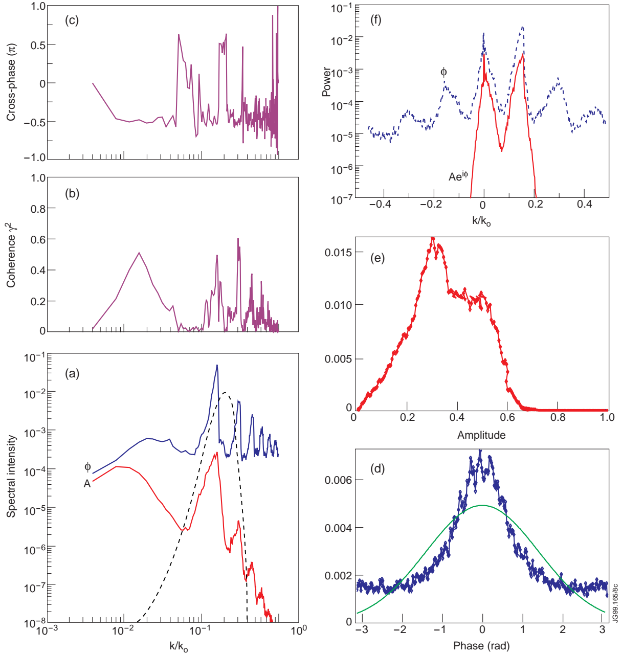
Fig.8: (a) Fourier spectra, (b) coherence, (c) cross-phase spectra of the simulation data of Fig.7, together with (d) phase pdf (e) amplitude pdf and (f) double-sided spectra.
