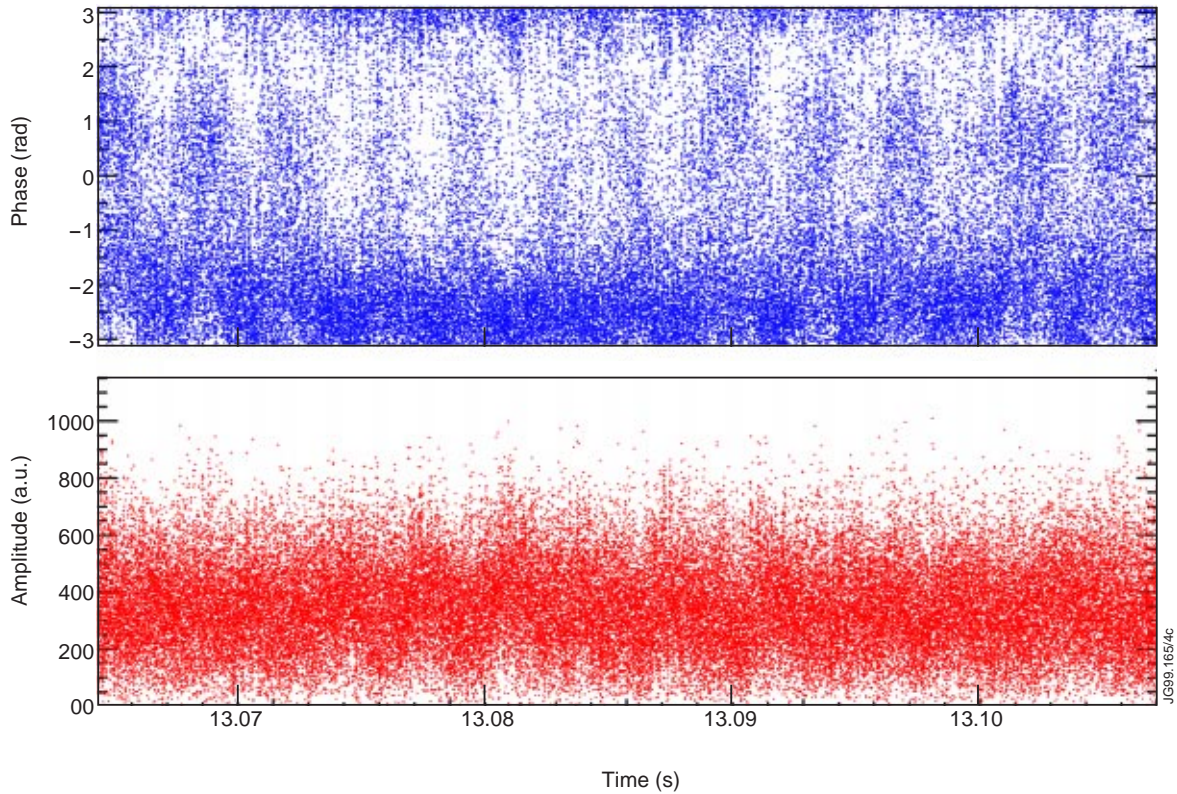
Fig.4: Expanded time sequence of phase and amplitude signals from shot #40477 using a 0.5\mu\text{s} sample period.
