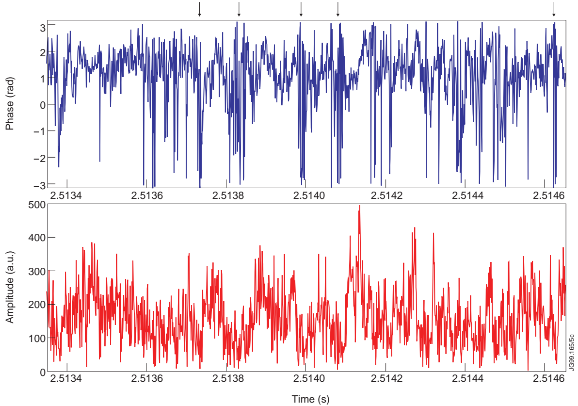
Fig.5: Raw phase and amplitude signals from the JET plasma core during the ohmic phase of an optimized shear discharge (shot #46270) using a 75GHz X-mode reflectometer. 1\mu\text{s} sample period.
