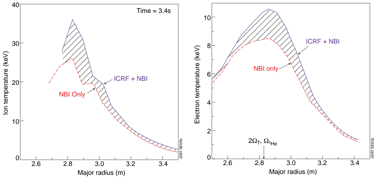
Figure 3. Ion and electron temperature profiles at 3.4s for the supershots shown in figure 2 with both NBI and NBI + ICRH.
