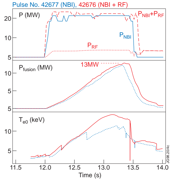
Figure 12. Sawtooth control with H-minority ICRH in a 3.8 MA hot ion H-mode which produced 13 MW of fusion power. A comparison NBI-only discharge suffered a large sawtooth crash at t = 12.7 \text{ s} which diminished the performance..
