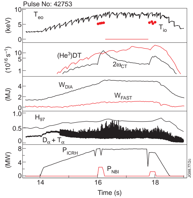
Figure 7. Plasma parameters for 8 MW of 2\omega_{\text{CT}} ICRH in JET. The neutron yield is 15% compared with \text{He}^3 minority heating which produces stronger bulk ion heating.
