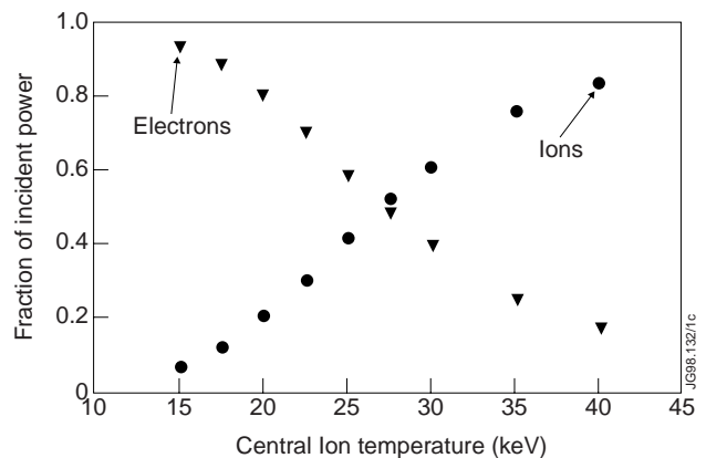
Figure 16. Ion temperature response to 1 MW of modulated mode conversion heating in TFTR.
