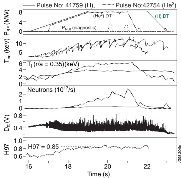
Figure 11. Hydrogen minority heating in a JET plasma with \text{D}:\text{T} = 8:92 giving a central electron temperature of 12 keV and an ion temperature of 7.5 keV.
