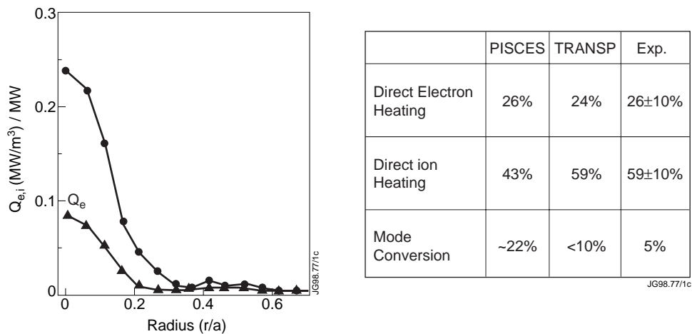
Figure 4. ICRH heating profiles determined by modulation techniques and comparison of total heating rates with theoretical calculations.
