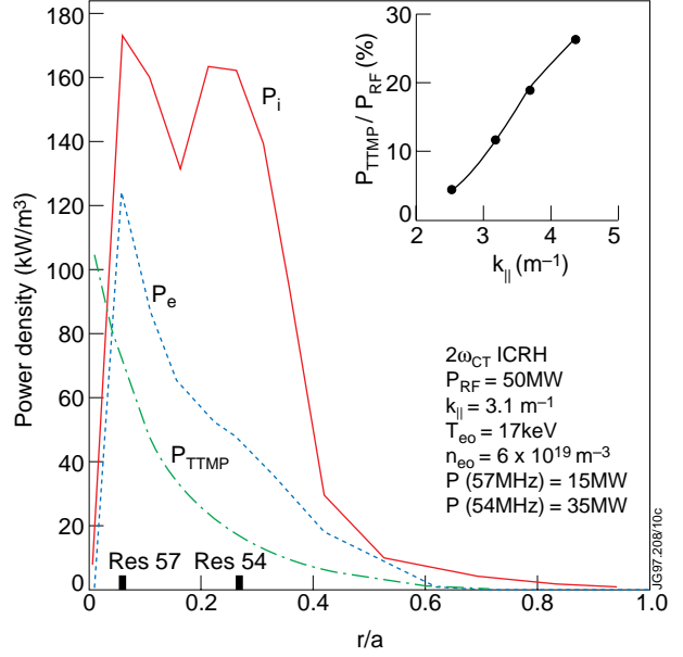
Figure 9. Heating profiles for the ITER ICRH case in figure 8. Two RF frequencies are used to broaden the heating profile. The inset shows the sensitivity of direct electron damping to k_{||} .
