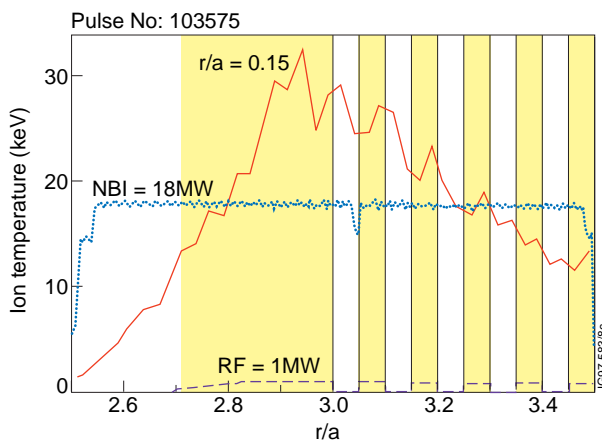
Figure 17. Strong ion heating by moded converted IBW is predicted by FELICE code at high T_i
