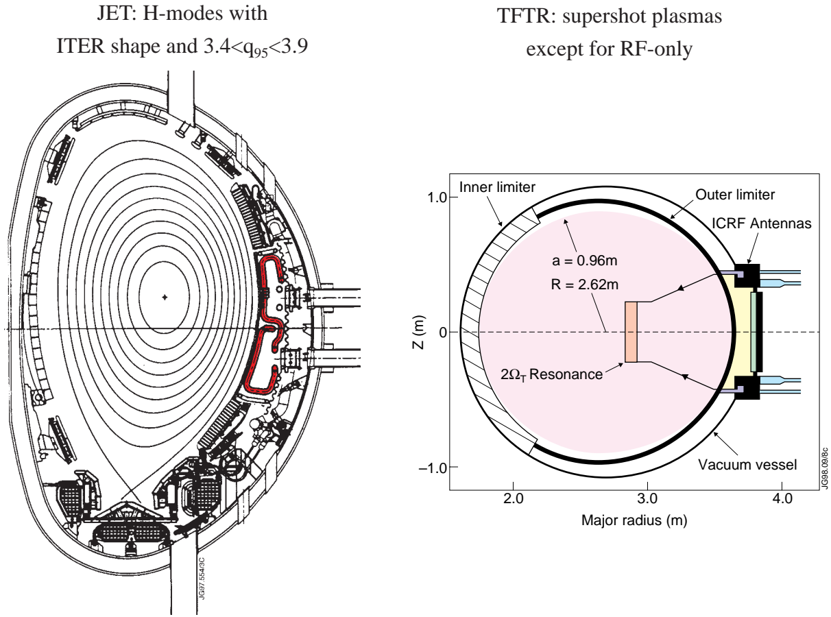
Figure 1. Poloidal cross sections of JET and TFTR showing the different plasma configurations used in the present experiment.
