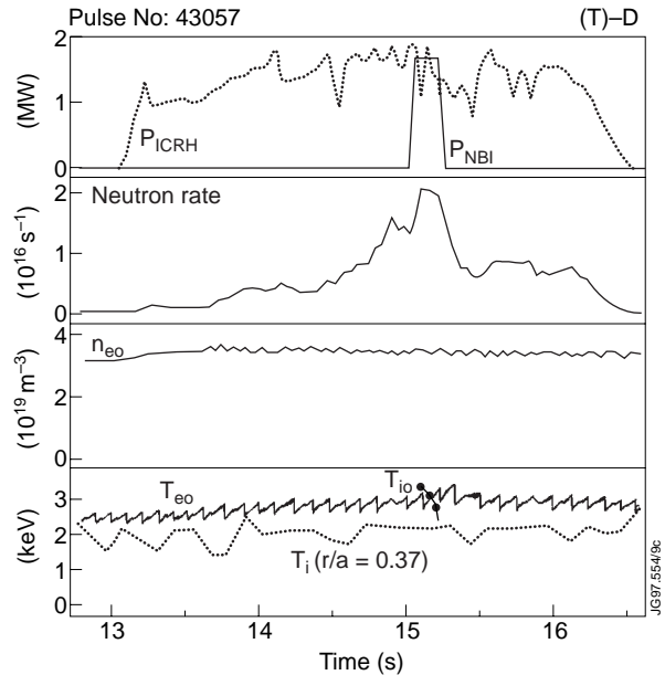
Figure 13. Suprathermal neutron production with (T)D ICRH.
