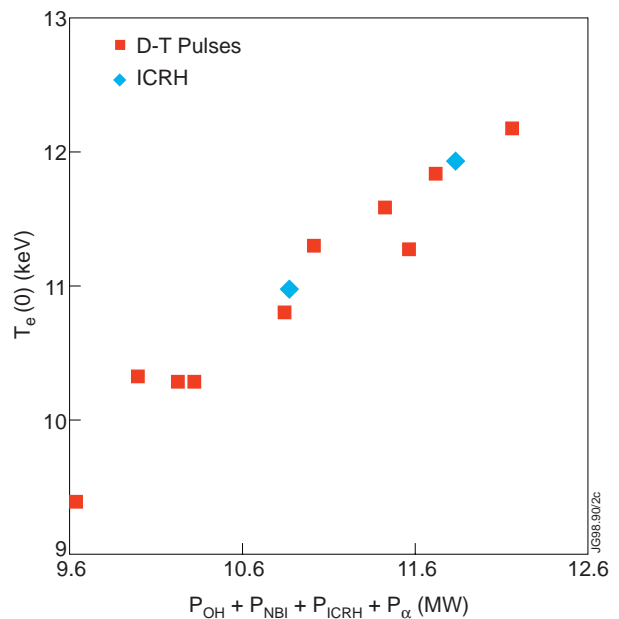
Fig. 3. Central electron temperature (ECE) versus total heating power, including alpha heating. The DT data (squares and star) and the ICRH emulation data (diamonds) are identified. The bars indicate the variation in NBI power compared to the 92% T pulse, 43011.
