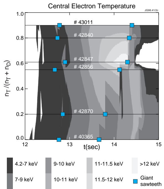
Fig. 2. A contour plot of central electron temperature against time (horizontal) and n_T/(n_T+n_D) (vertical) for the six pulses of the alpha heating scan.. Giant sawteeth are marked with squares.
