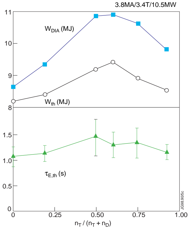
Fig. 5. (top) Diamagnetic and thermal energy contents with (bottom) the plasma energy confinement time versus DT mixture.
