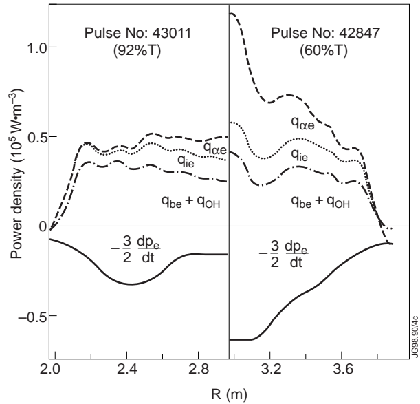
Fig. 4. Electron power density profiles for pulse 43011, inside the magnetic axis, and pulse 42847 outside. Beam electron plus Ohmic heating, ion-electron equipartition and alpha heating are shown. The electron heating rate appears negated for clarity.
