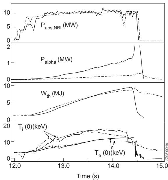
Fig. 1. Traces of (a) absorbed NBI power, (b) alpha heating power, (c) thermal plasma energy content and (d) central ion (CXs) and electron temperatures (ECE) for pulse 42847(solid), which had the largest fusion output of the scan, and pulse 43011(dashed), which had the largest tritium content.
