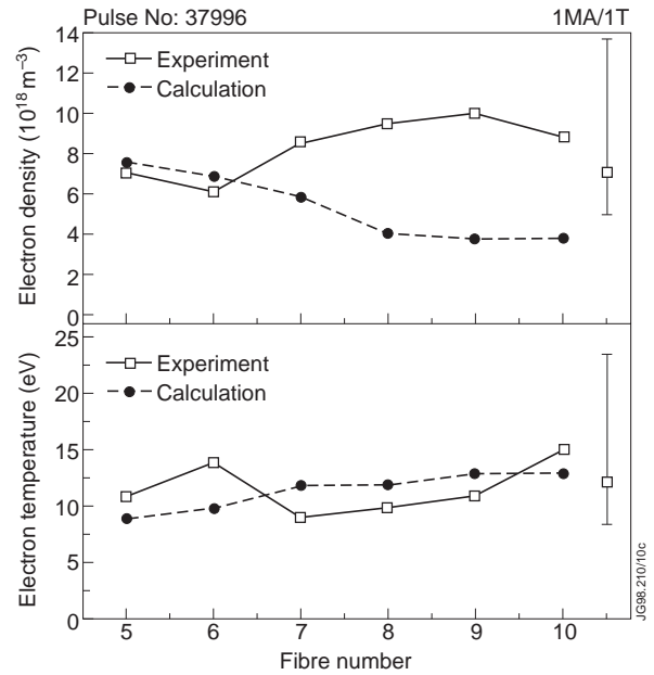
Fig.6 Comparison of n_e and T_e values derived from measured and calculated He I line ratios, for the ohmic pulse 37996.
