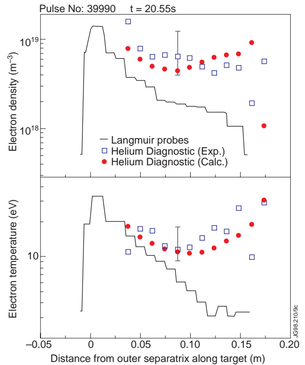
Fig.8 Comparison of experimental n_e and T_e profiles measured with Langmuir probes at the outer target plate (straight line) with values derived from measured and calculated He I line ratios, for H-mode pulse 39990.
