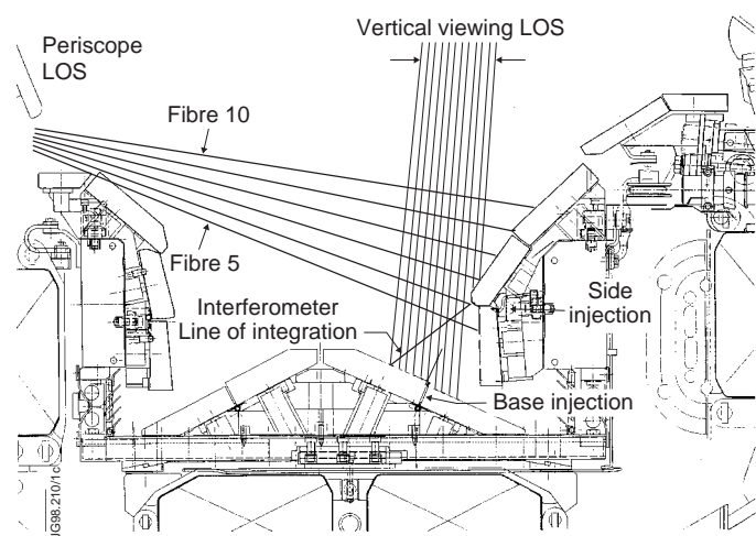
Fig.1 Viewing arrangement for the thermal helium diagnostic in the JET MkIIa outer divertor leg.
