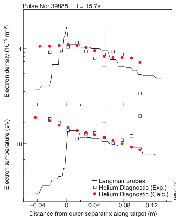
Fig.5 Comparison of experimental n_e and T_e profiles measured with Langmuir probes at the outer target plate (straight line) with values derived from measured and calculated He I line ratios, for the ohmic pulse 39885.
