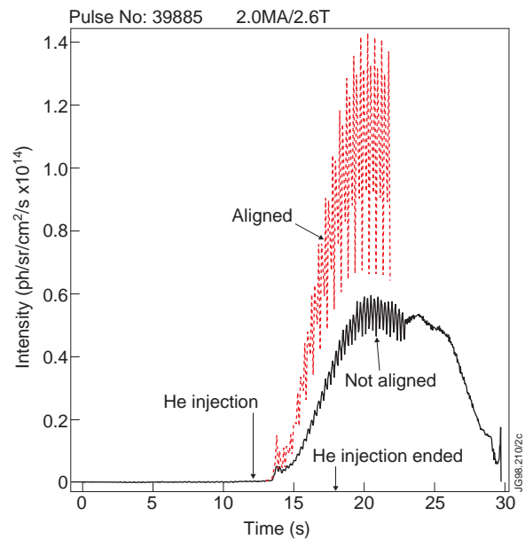
Fig.2 HeI, \lambda=667.8nm , intensity measured with the vertically viewing spectrometer and with the interference filter, in the ohmic pulse 39885.
