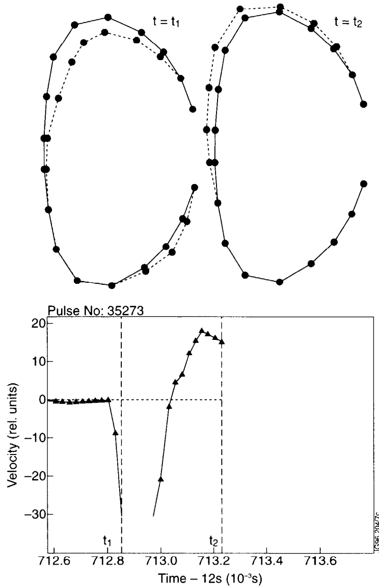
Fig. 7 Velocity of the main plasma perpendicular to the vessel (dashed line) at two different times during an ELM measured by an array of magnetic probes (solid line), the same ELM as in fig. 5 is shown
