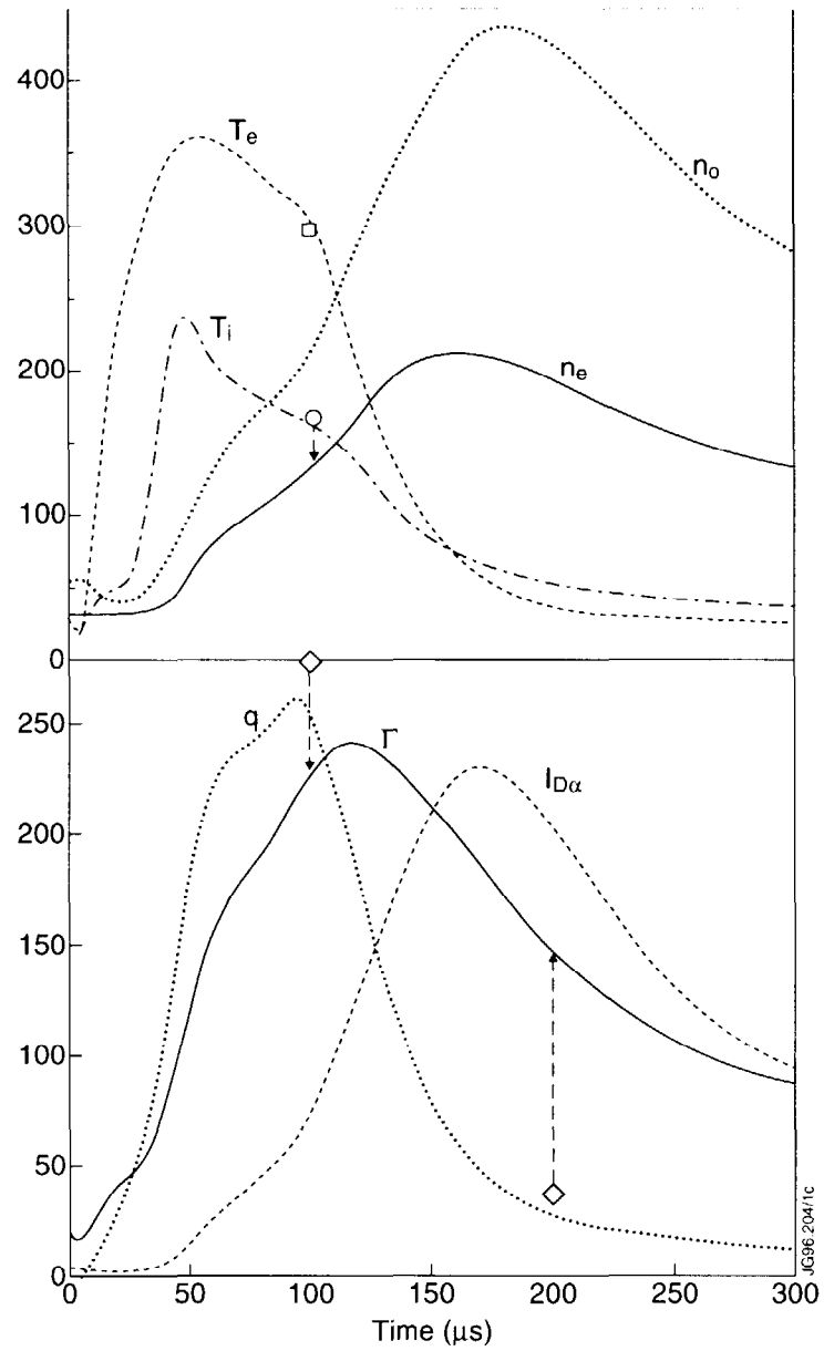
Fig. 1 Calculated evolution of plasma parameters at the target plate during an ELM ( T_e , T_i in eV, n_e in 10^{18} \text{ m}^{-3} , n_0 in 10^{17} \text{ m}^{-3} , q in 50 \text{ MW}\cdot\text{m}^{-2} , \Gamma in 10^{23} \text{ m}^{-2}\text{s}^{-1} , I_{D\alpha} in rel. units) o - n_e , \square - T_e , \diamond - \Gamma for case \Delta N = 0
