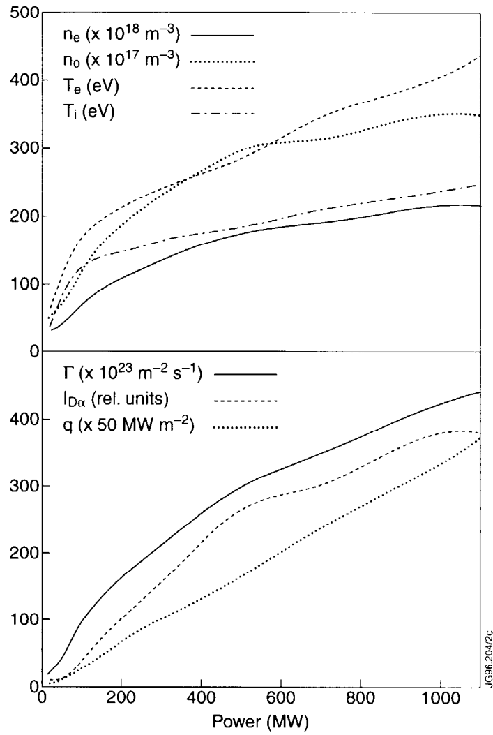
Fig. 2 Calculated dependence of the plasma parameters at the target plate on the released power ( \delta t = 100 \mu\text{s} ), \Delta N = 0
