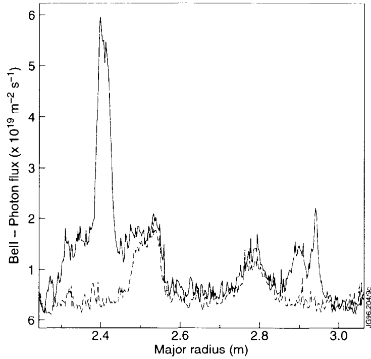
Fig. 3 Be II photon flux before (dashed line) and during (solid line) an ELM as a function of the major radius ( \lambda = 527 \text{ nm} , \delta\lambda = 1 \text{ nm} , Be target plate, shot 34953)
