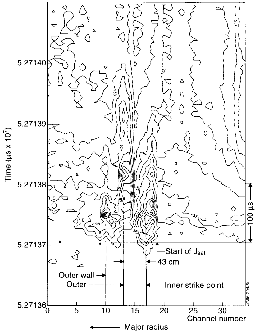
Fig. 6 Contour plot of the soft X - ray intensity in the divertor region during the same ELM as in fig. 5 as a function of time
