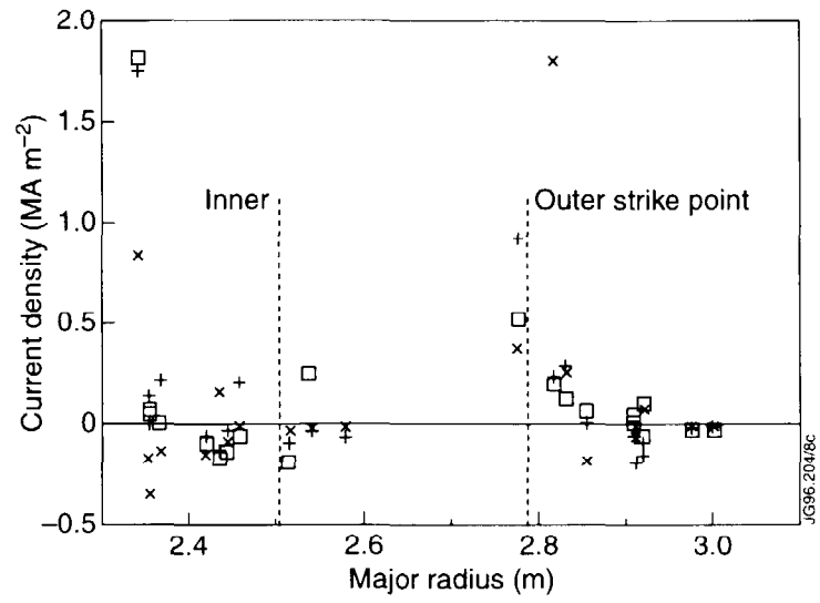
Fig. 8 Current density profile at the divertor plate during three different ELMs (shots 34955,34957), each symbol represents data from a different ELM
