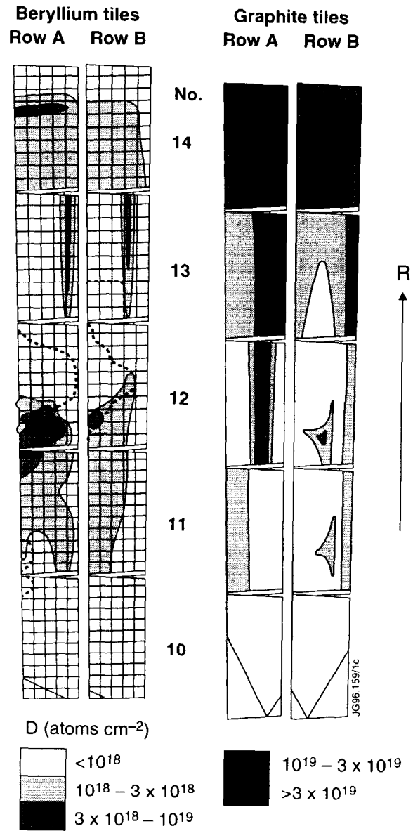
Figure 3: An overall view of the amounts of D retained on the outer floor tiles of one support bar after operations using graphite tiles, alongside a comparable view for the Be tiles.
