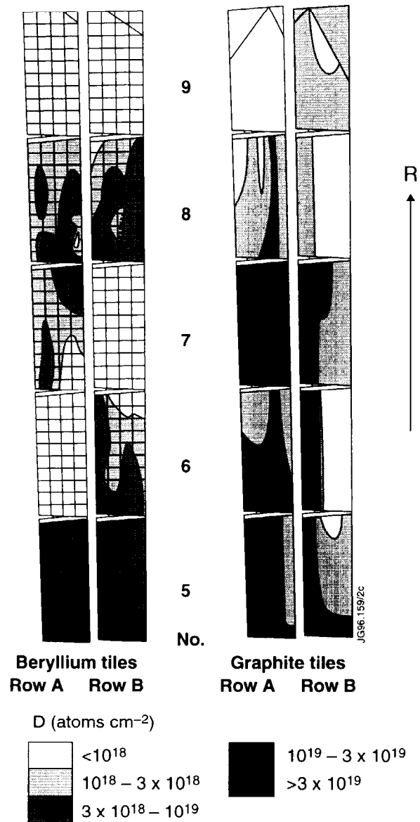
Figure 4: An overall view of the amounts of D retained on the inner floor tiles of one support bar after operations using graphite tiles, alongside a comparable view for the Be tiles.
