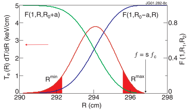
Figure 8: Integrand of Eq. 5 and the function F defined in Eq. 6, along with the values R^{\min} and R^{\max} for g = 0.9 . The shadowed area corresponds to 10 % of the total emission.
