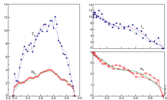
Figure 4: The same as in Figure 3 but with the profiles shifted by 10 cm in major radius.
