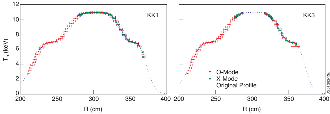
Figure 13: Simulated electron temperature profiles for KK1 and KK3 diagnostics with the original profile for the Pulse No: 47413. The error bars correspond to the spatial resolution of Figure 12.
