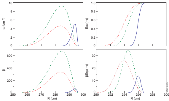
Figure 7: From top to bottom. Local absorption, emission, transmission and emitting coefficients versus the major radius for the parameters of Table 2: cases 1 Pulse No: 47413 (dotted), 2 (solid), and 3 (dashed).
