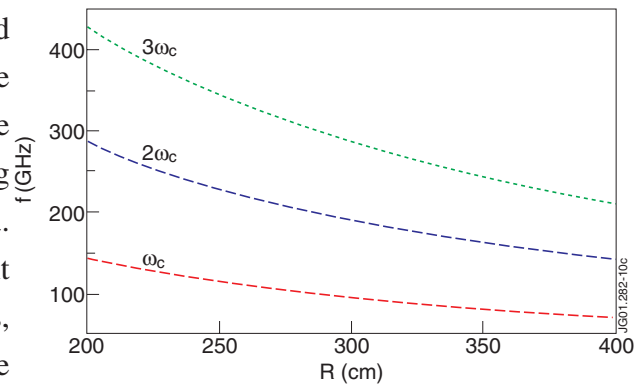
Figure 10: Radial dependence of the different cyclotron harmonics for the Pulse No: 47413.
