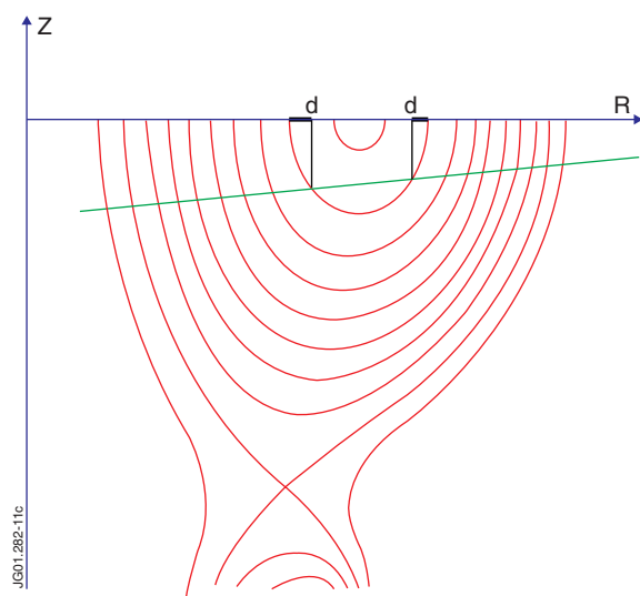
Figure 11: Sketch of the difference between the major radius and the equivalent radius corresponding to the flux surfaces
