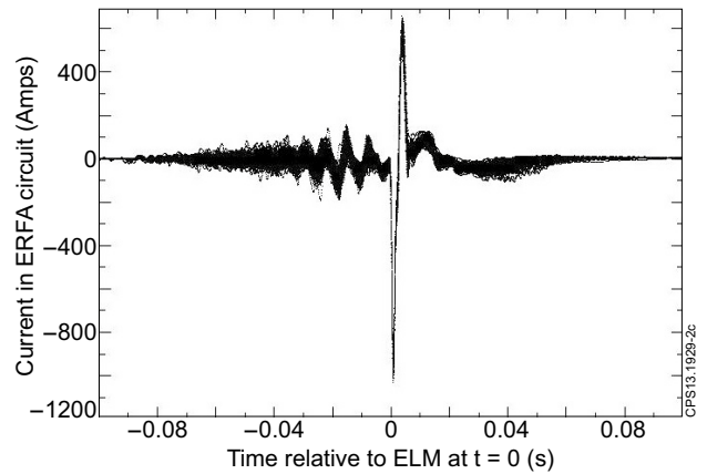
Figure 4: The current (Amps) in the ERFA vertical control system measured between the start of the (n - 1) th ELM and the start of the (n + 1) th ELM, with time offset so that the n th ELM appears at t = 0 , is averaged over all ELMs in a pulse and simultaneously plotted for all pulses in our 120 pulse dataset.
