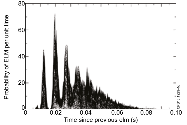
Figure 2: The ELM waiting time pdf inferred from analysing 120 pulses and combining the data to form a single pdf. Each line corresponds to data from an additional pulse.
