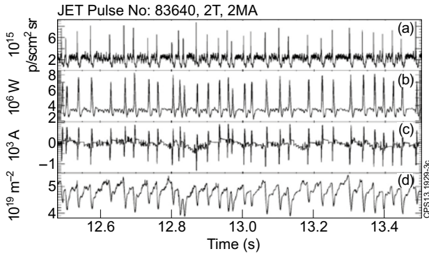
Figure 1: Signals from a typical pulse (83640) in the set 83630–83794. The signals shown are: Be II radiation (a), the total radiated power (b), the current in the EFRA vertical control system (c), and the line integrated edge density (d). The ELMs are associated with a strongly peaked Be II and radiated power (signals (a) and (b)), a rapid response of the vertical control system to keep the plasma stable (c), and a drop in the edge density (d).
